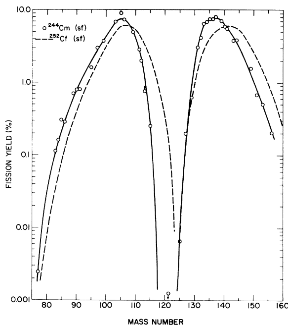
FIG. 1. Mass-yield curve for the spontaneous fission of ^{244}\text{Cm} compared with that for spontaneous fission of ^{252}\text{Cf} . Postneutron masses are shown.
