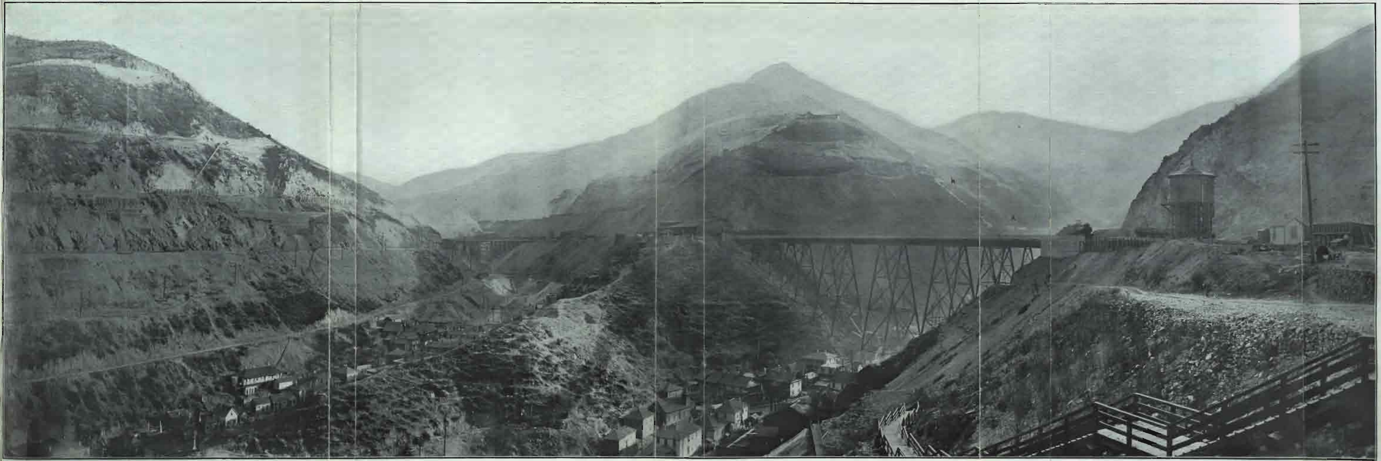
GENERAL VIEW OF THE UTAH COPPER COMPANY'S MINING PROPERTY AT BINGHAM SHOWING THE NORTHERLY SIDE OF THE MOUNTAIN UPON WHICH STEAM SHOVEL OPERATIONS ARE BEING CONDUCTED. THE STEAM SHOVELS ARE SEEN AT WORK ON THE WESTERLY SLOPE OF THE MOUNTAIN IN BINGHAM CANYON, AND THE SYSTEM OF SWITCHBACKS IN CARR FORK CANYON, THAT EXTENDS FROM THE BINGHAM YARD TO THE TOP OF THE MOUNTAIN, IS SHOWN ON THE RIGHT. IN THE FOREGROUND IS SEEN THE STEEL VIADUCT OF THE BINGHAM AND GARFIELD RAILWAY ACROSS CARR FORK CANYON. THIS VIADUCT HAS A LENGTH OF 690 FEET AND THE MAXIMUM HEIGHT OF 190 FEET.
