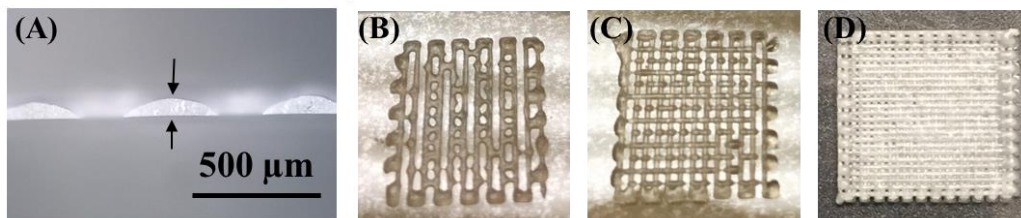
Figure 3.2 Determining layer height and dwell time on 10 \times 10\ \text{mm}^2 scaffolds. (A) Cross-sectional view of the C3 filament measuring \sim 75\ \mu\text{m} in height, (B) Second layer printing with zero dwell time, (C) Second layer printing with 1 min dwell time, and (D) Second layer printed with 2.5 min dwell time
