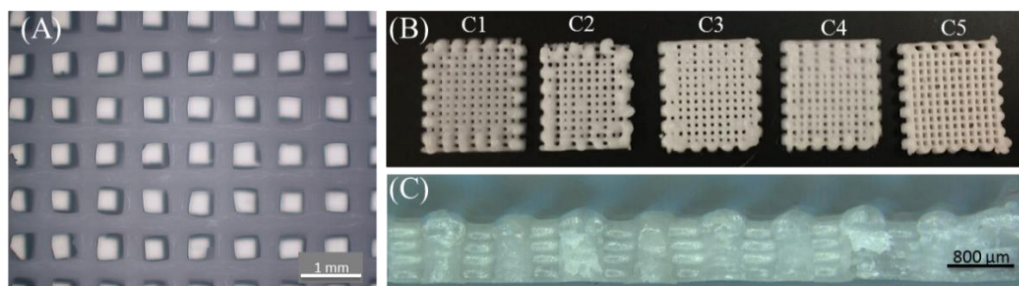
Figure 3.9 Micro- and macroscopic images of PCL/45S5 composite scaffolds. (A) Optical microscopic image showing the pores ( \sim 160 \mu\text{m} ) in a composite scaffold fabricated with C5 paste. (B) Scaffolds fabricated with different composite pastes (C1 to C5). (C) Cross section of C5 scaffold.
