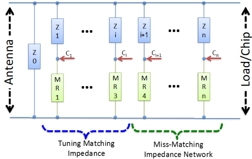
Figure 3.1. Proposed Impedance Matching Network for RFID lanes with memristors that have impedance. Z_i and Z_n denotes bias impedances for each lane. M R_i denotes the memristor for each lane, and C_n is the control signal for lane.
