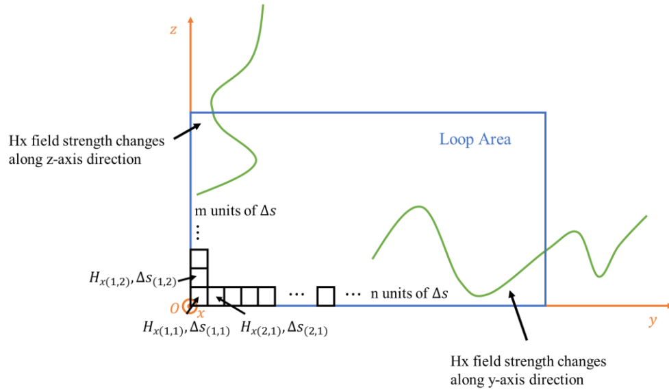
Figure 3.17 Schematic of approximate voltage calculation
