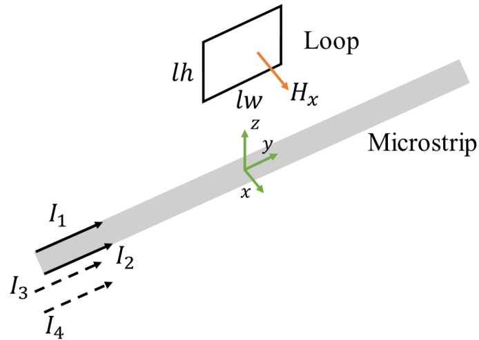
Figure 3.5 Schematic of analytical probe model
