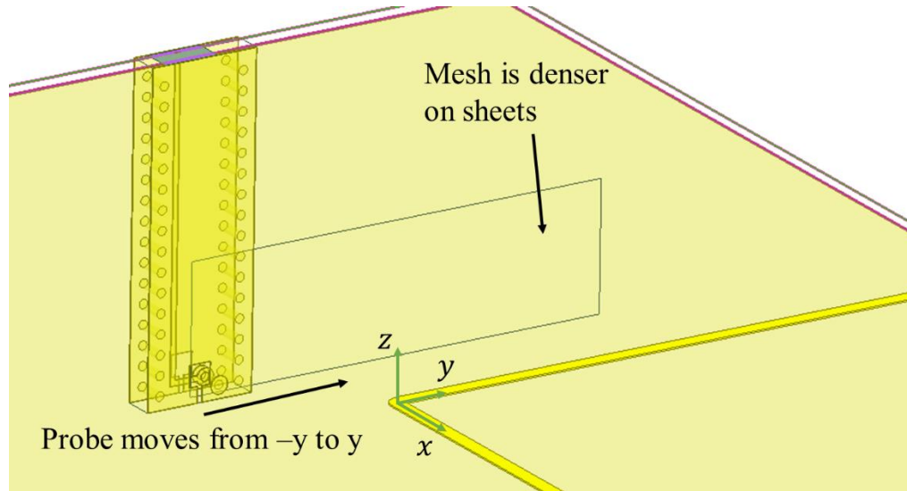
Figure 4.4 Simulation model of bend microstrip and probe
