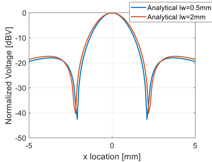
Figure 3.11 Comparison of analytical results between different loop width
