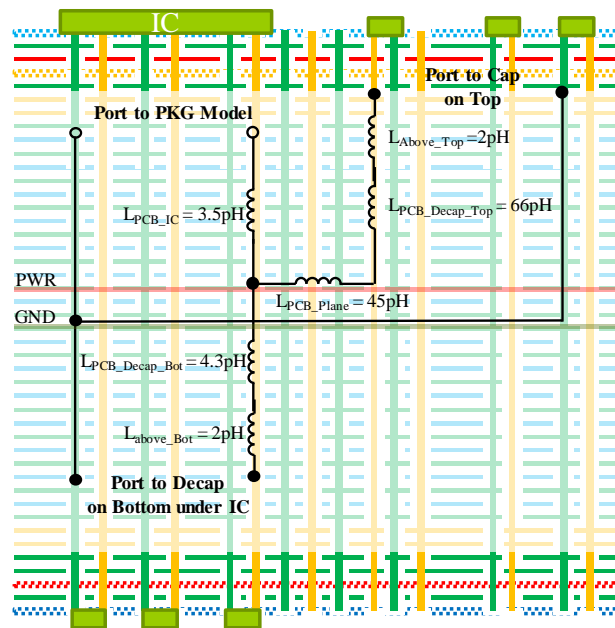
Figure 14. Equivalent Circuit Model Extraction for PCB
