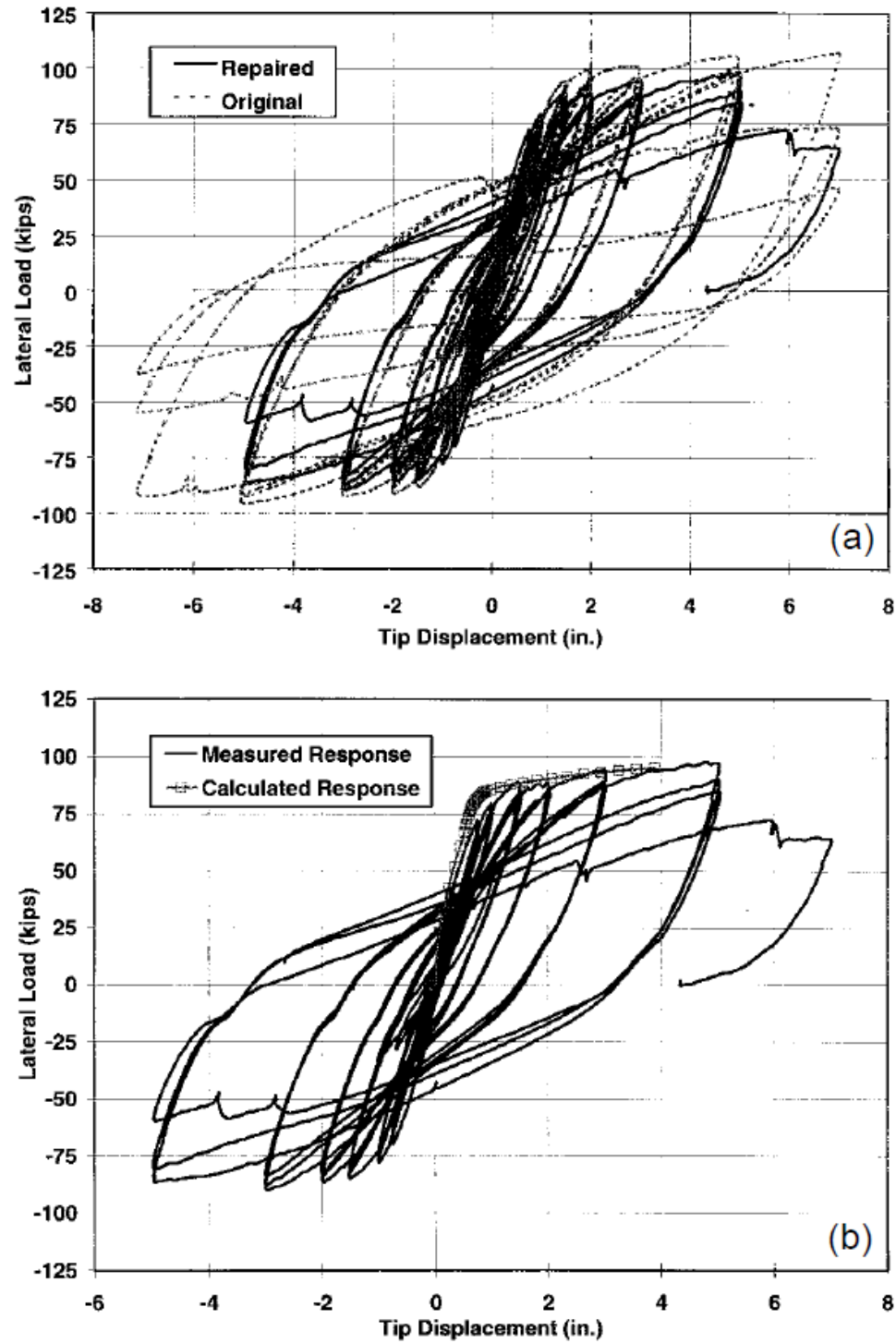
Figure 2.11 - Force-Displacement Response of 430SR Compared to: (a) 430S; and (b) Theoretical Response (Lehman, et al., 2001) (1 kip = 4.448 kN, 1 in. = 25.4 mm)
