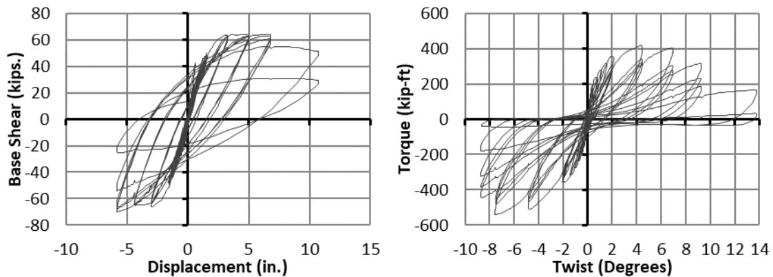
Figure 3.6 - Calt-2 Experimental Results; Shear-Displacement (left) Torque-Twist (right) (1 kip = 4.448 kN, 1 kip-ft = 1.356 kN-m, 1 in. = 25.4 mm)
