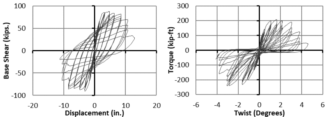
Figure 3.5 - Calt-1 Experimental Results; Shear-Displacement (left) Torque-Twist (right) (1 kip = 4.448 kN, 1 kip-ft = 1.356 kN-m, 1 in. = 25.4 mm)
