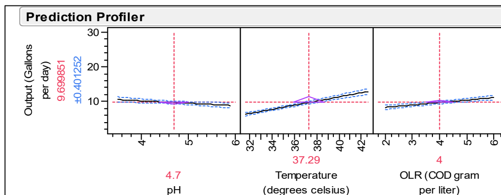
Figure 15. Prediction Profiler
