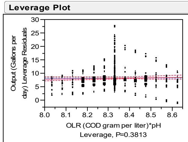
Figure 21. Leverage Plot for pH & OLRs vs Biogas Production
