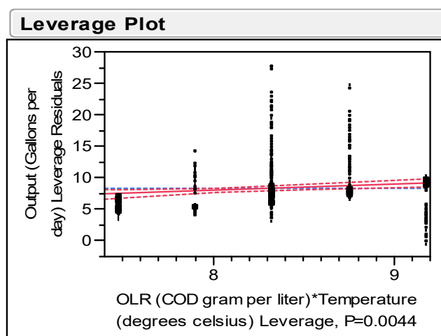
Figure 20. Leverage Plot for Temperature & OLRs vs Biogas Production
