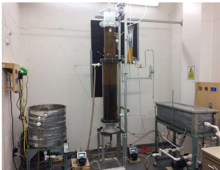
Figure 6. Two-Stages Expanded Granular Sludge Bed Reactor System
