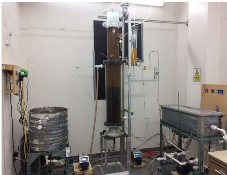
Figure 3. Two-Stages Expanded Granular Sludge Bed Reactor System
