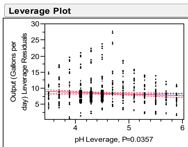
Figure 16. Leverage Plot for pH vs Biogas Production
