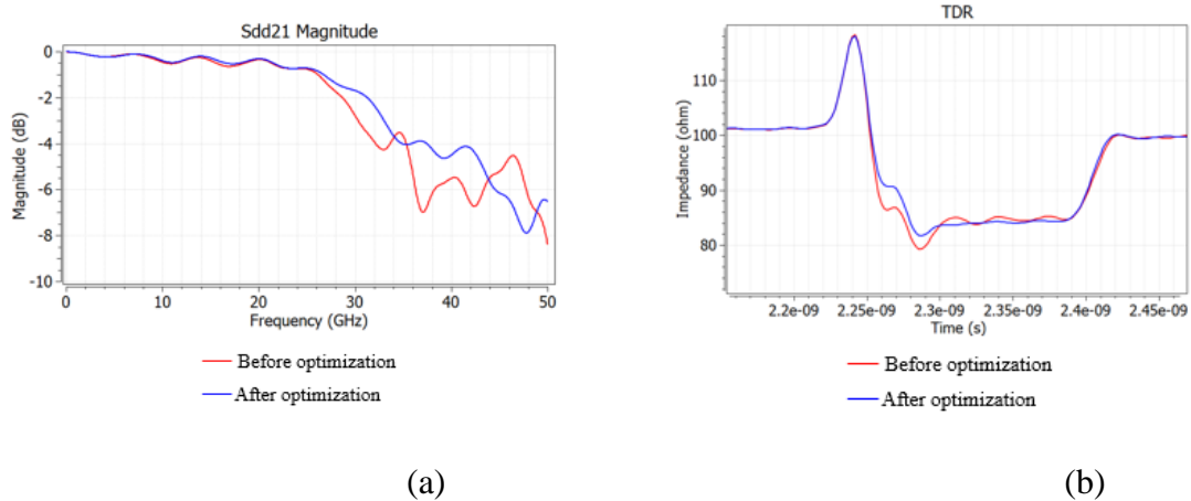
Figure 3.28. Simulation results comparison for insertion loss and TDR ;(a) Sdd21 magnitude comparison; (b) TDR result comparison.
