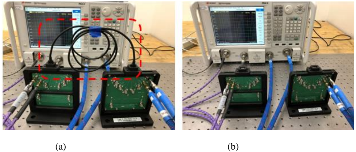
Figure 2.10. S-parameter measurement setup for total structure and 1X open.
