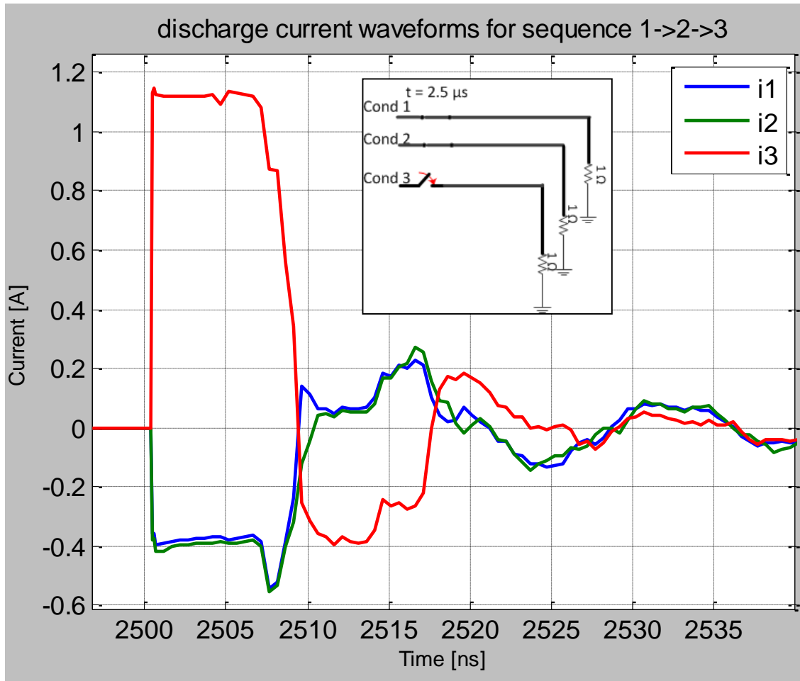
Figure 4.25. Discharge current on conductors 1 to 3 during the discharge of conductor 3 at 2.5 \mu s.
