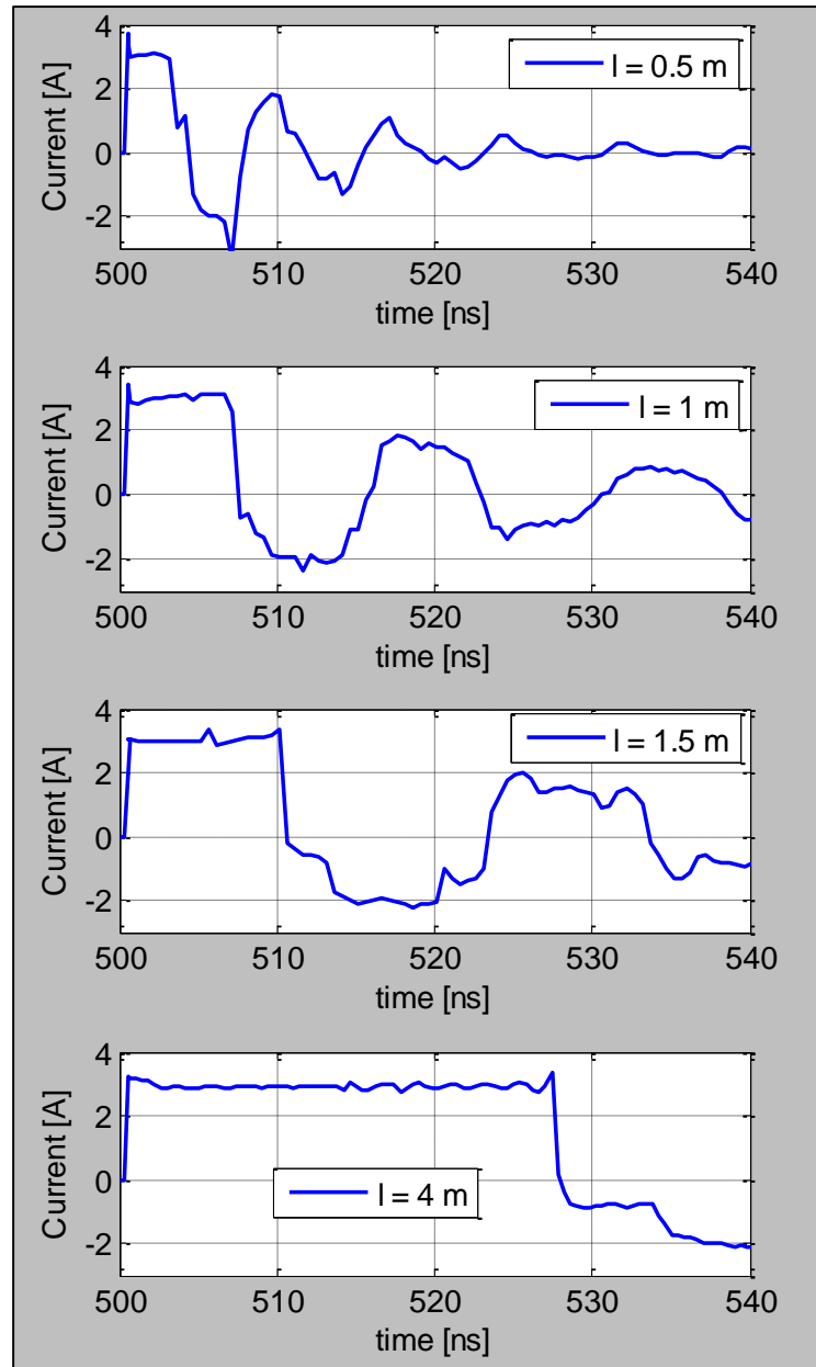
Figure 4.30. The effect of cable length on the pulse length of the discharge current waveform
