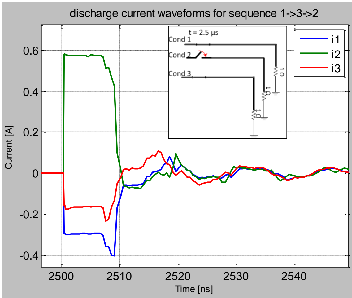
Figure 4.27. Discharge current on conductors 1 to 3 during the discharge of conductor 3 at 2.5μs.
