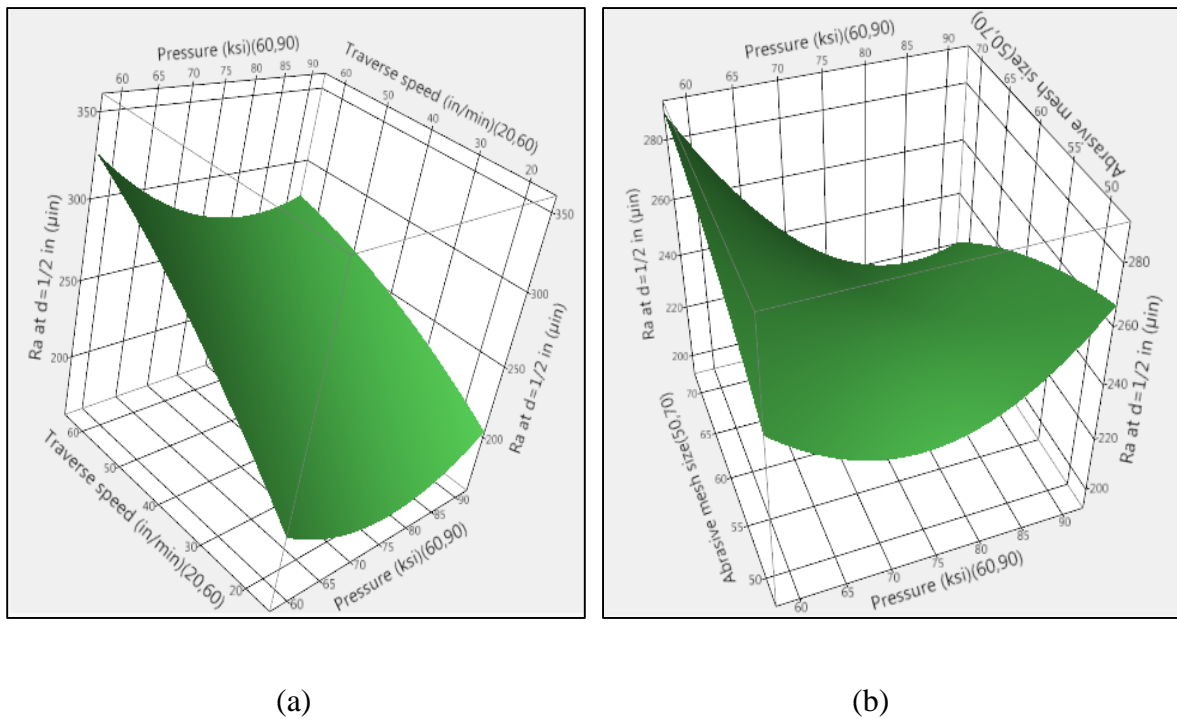
Figure 5.9. Response surface plots showing the effect of variables a) pressure and traverse speed b) pressure and abrasive mesh size c) traverse speed and abrasive mesh size on Ra at a depth of \frac{1}{2} " at an AFR of 1.5 lb/min
