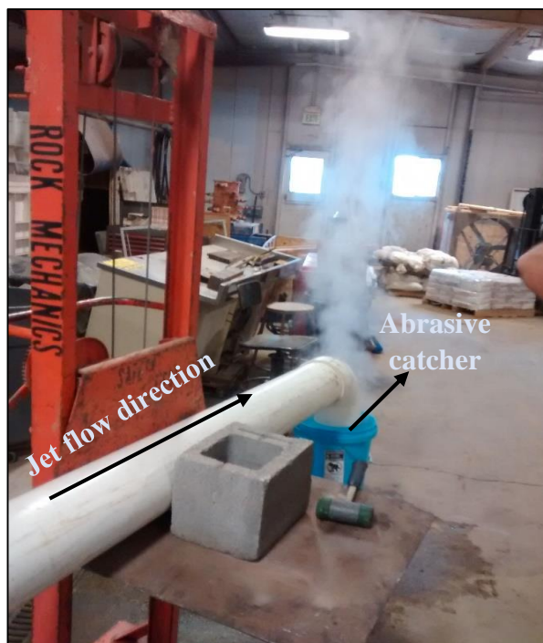
Figure 4.11. Abrasive capture after jet exit
