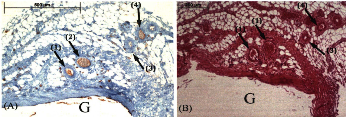
Figure 15. CD31 (A) and H&E (B) stained section of 93B3-0 after 4 weeks in a rat. A sample of 4 blood vessels selected and identified by arrows with assigned numbers. Brown in CD31 section shows platelets or endothelial cells. CD31 identified that these are blood vessels because they stained brown. This confirms that the regions marked with black arrows in the H&E stained section are indeed blood vessels. G= Unreacted (decalcified) Glass.
