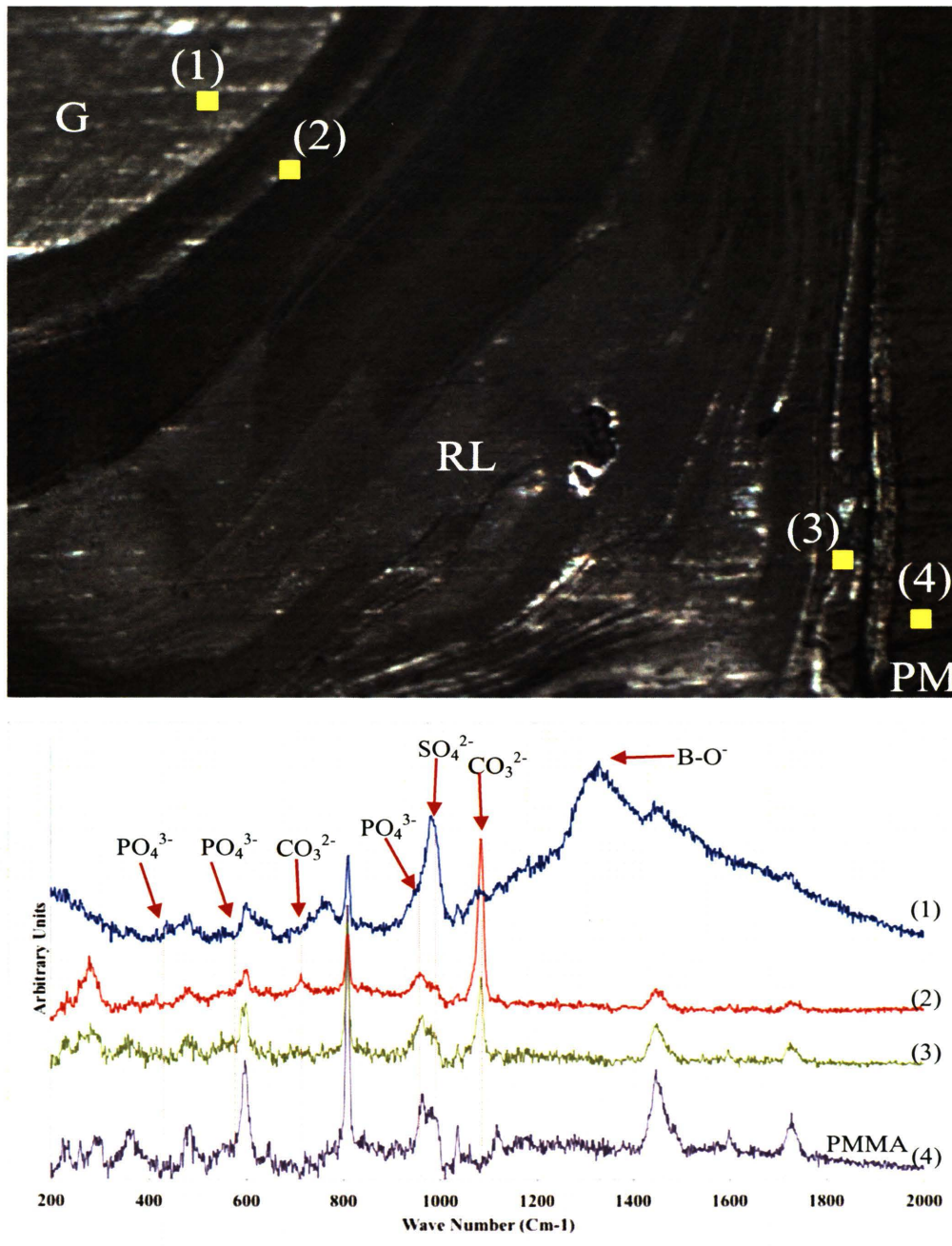
Figure 4. Optical micrograph (10X) of the polished cross-section of the CaLB-12 implanted subcutaneously in a rat for 12 weeks (A). Micro-Raman spectra (B) were collected for the point showed with squares. Carbonate ion ( \text{CO}_3^{2-} ) has 2 peaks at 711 \text{ cm}^{-1} and 1085 \text{ cm}^{-1} . Phosphate ion ( \text{PO}_4^{3-} ) represents HA which has 3 major peaks at 420 \text{ cm}^{-1} , 570 \text{ cm}^{-1} , and 960 \text{ cm}^{-1} . The sulfate ion ( \text{SO}_4^{2-} ) has a primary peak at 1000 \text{ cm}^{-1} . G: Unreacted Glass, RL: Reacted Layer, PM: PMMA, HA: Hydroxyapatite
