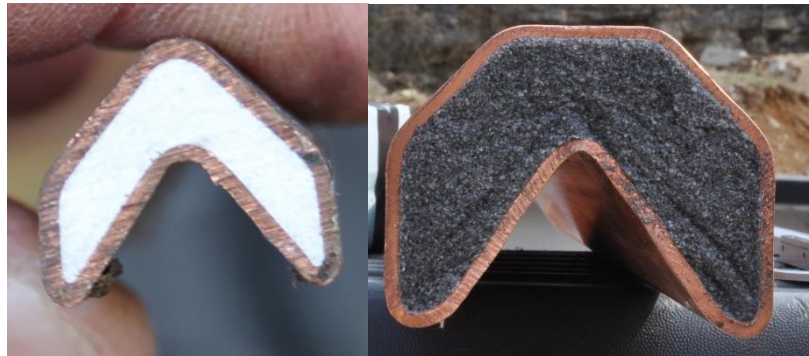
Figure 2-4. Typical LSC (left) 10,500 gr/ft. LSC (right).
