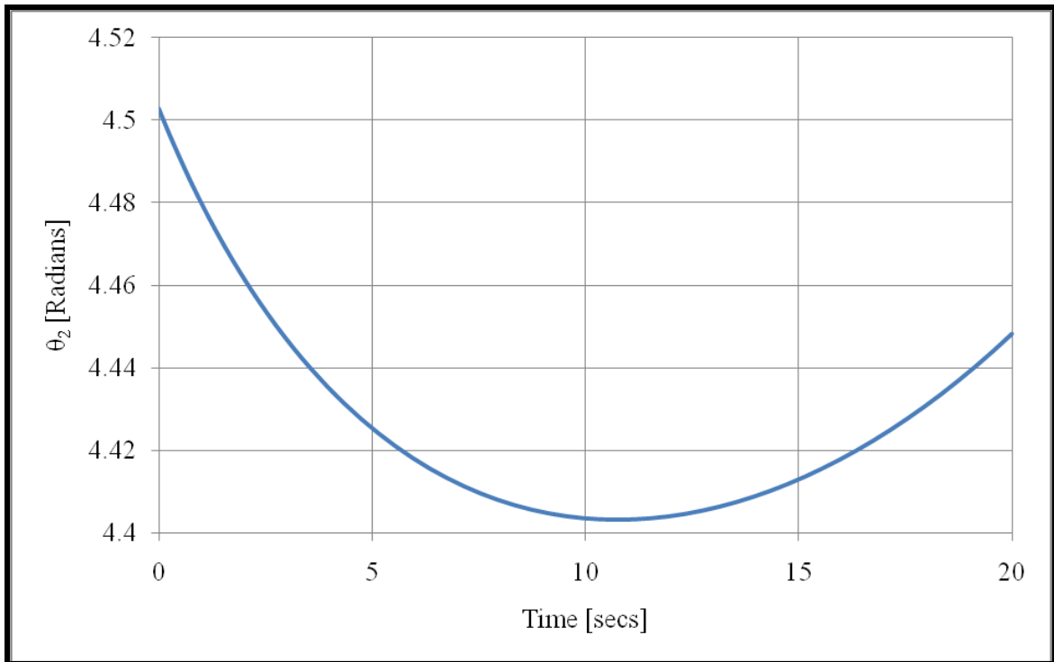
Figure 5.6 Clamshell Dredge Simulation Kinematics Results I
