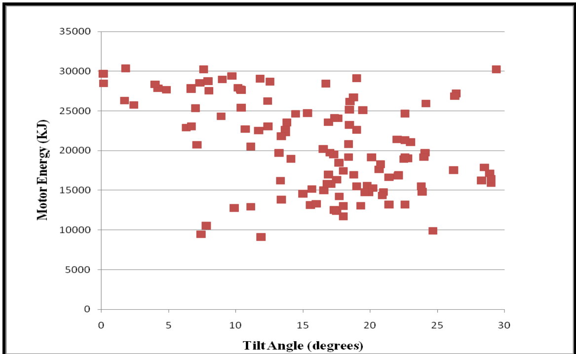
Figure 5.3 Motor energy (kJ) against average tilt angle (degrees)
