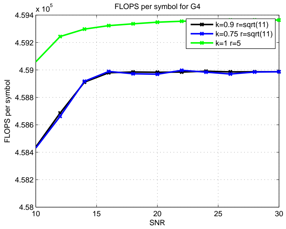
Figure 5.8 Complexity of G4
