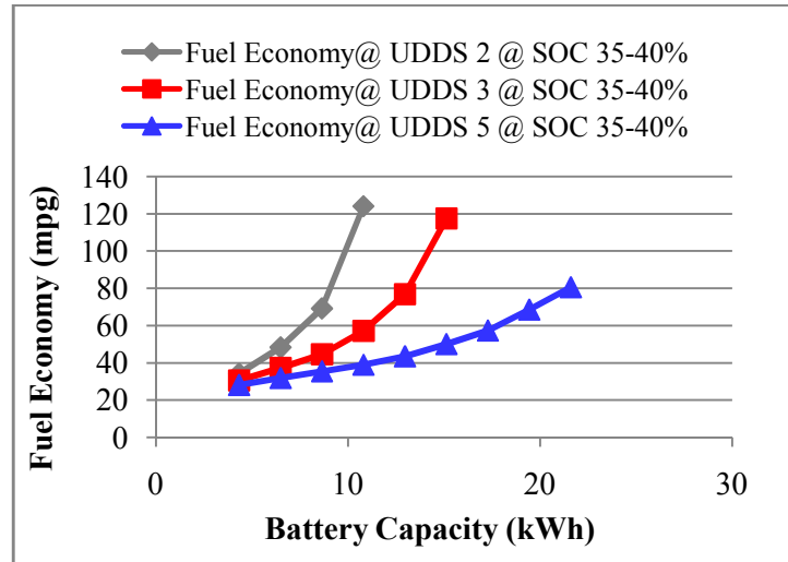
Figure 3.7. Fuel economy vs. battery capacity for different drive cycles
