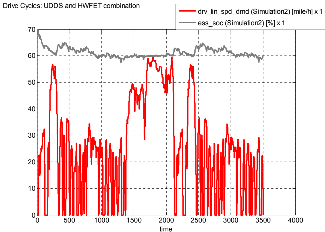
Figure 2.10. Load follower control strategy for combined driving cycle
