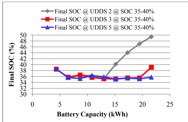
Figure 3.8. Final SOC vs. battery capacity for different drive cycles
