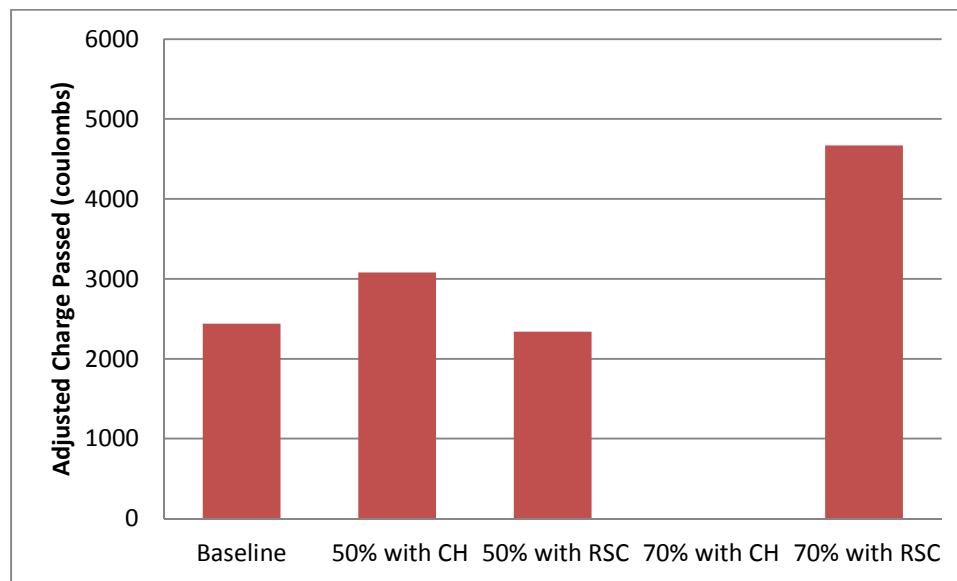
Figure 4.19. Rapid Chloride Permeability Results for 1-3 Mixtures
