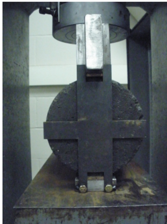
Figure 3.10. Splitting Tensile Testing Jig
