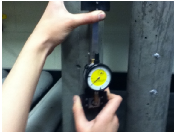
Figure 3.12. DEMEC Gauge and Specimen
