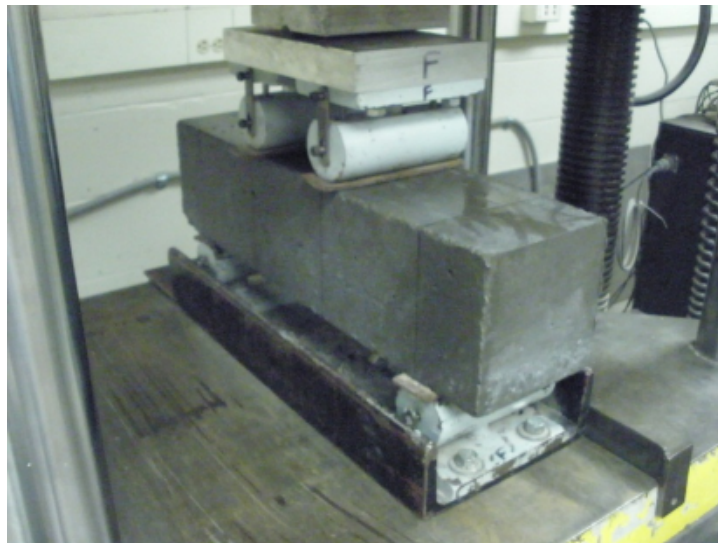
Figure 3.7. Beam Testing Apparatus
