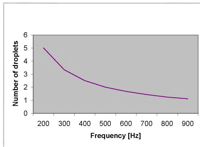
Figure 4: Predicted number of droplets released at 20% duty cycle
