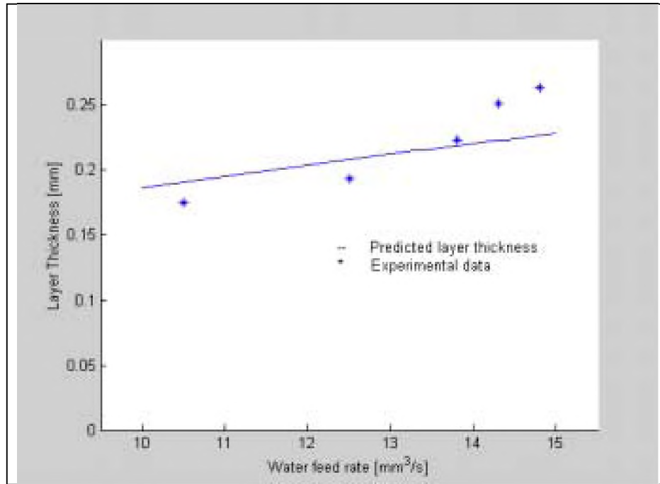
Figure 5: Comparison of predicted to measured layer thickness
