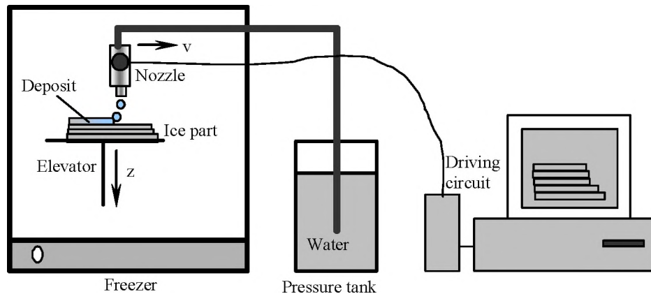
Figure 1. Principle of Rapid Freeze Prototyping
