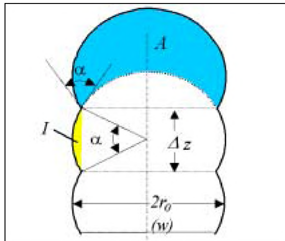
Figure 3: Cross section illustration of an ice line
