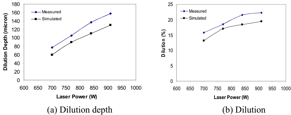
Figure 5-Dilution depth and dilution as a function of laser power for travel speed of 20 ipm and powder mass flow rate of 4.68g/min for laser deposited Ti-6Al-4V
