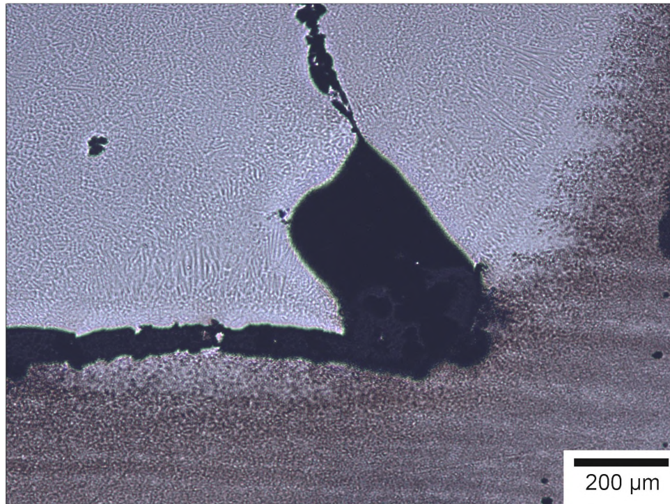
Figure 6: Corner void
