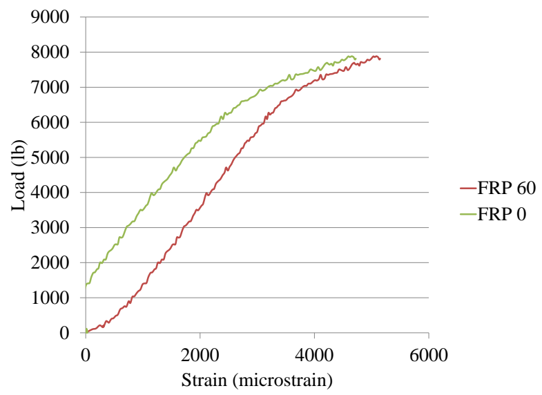
Figure 3.11. Load-Strain: FRP 60,0 #3
