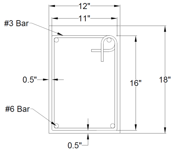
Figure 4.2. Stirrup Dimensions
