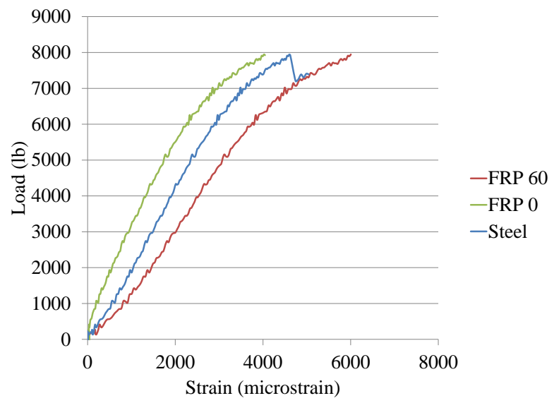
Figure 3.10. Load-Strain: FRP 60,0 #2
