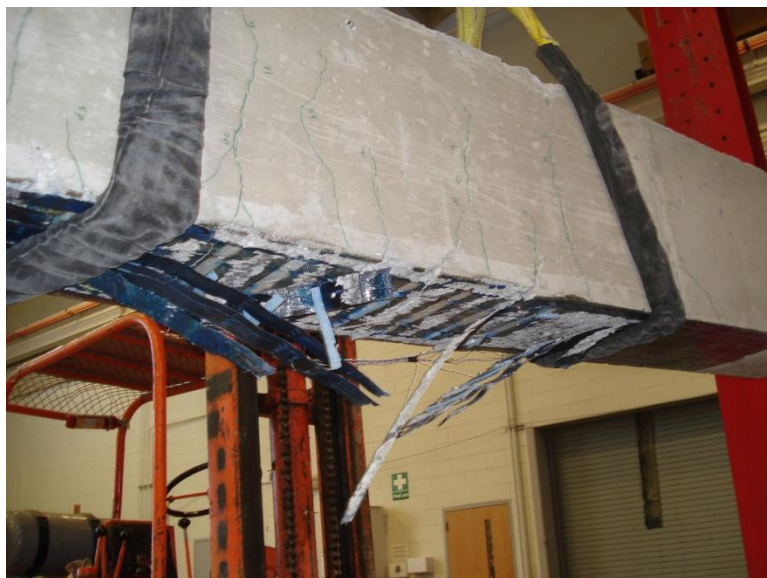
Figure 4.61. Failure of Beam 9
