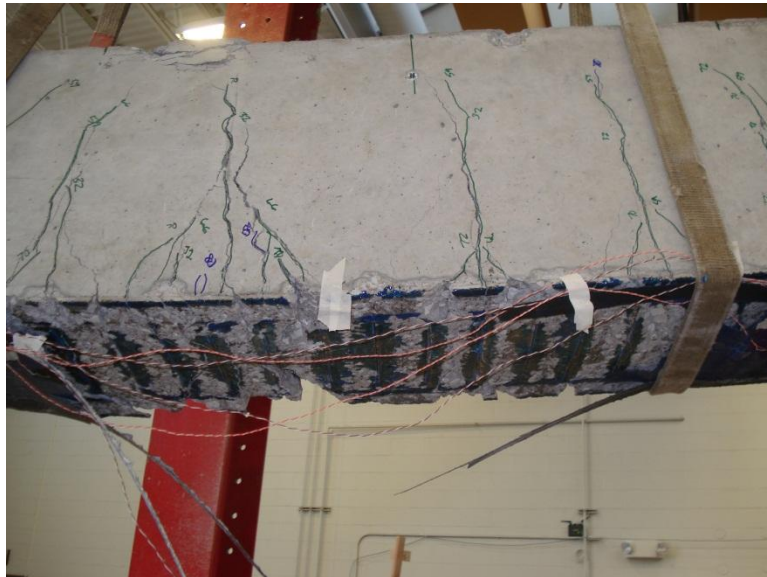
Figure 4.13. Failure of Beam 2
