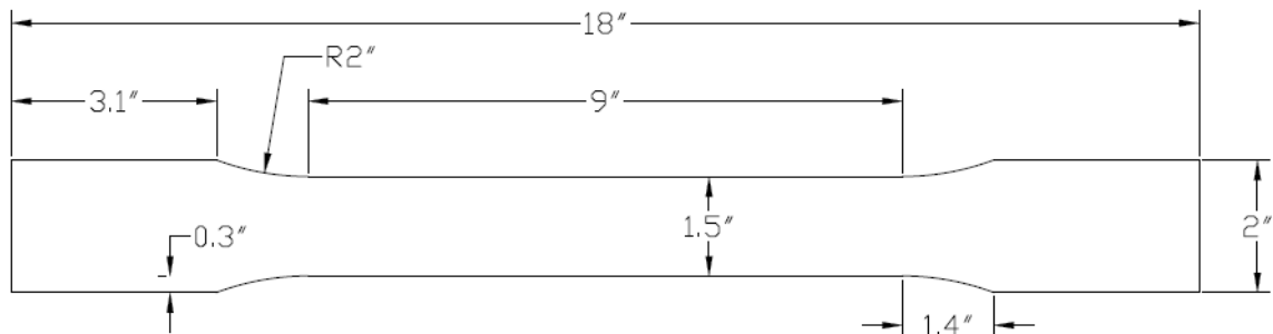
Figure 3.1. Coupon Dimensions
