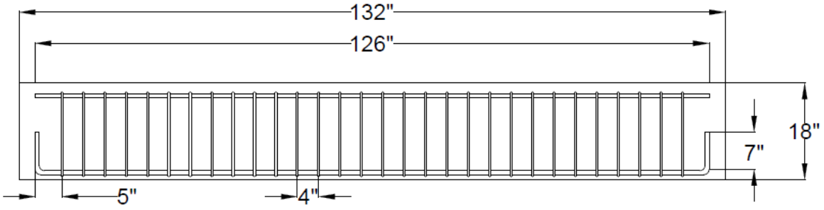
Figure 4.1. Beam Dimensions
