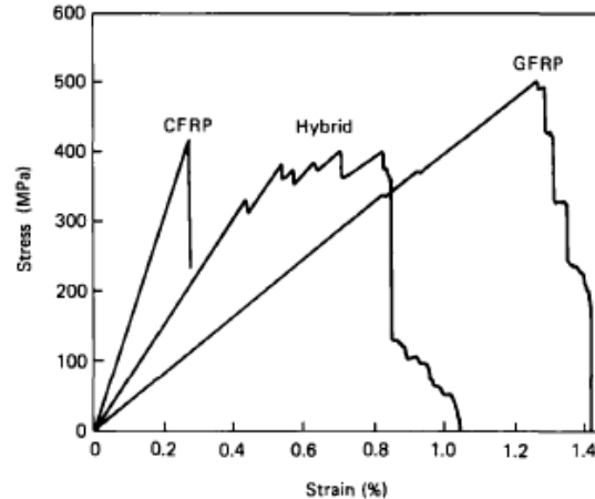
Figure 2.1. Typical Load Strain Curves for Carbon, Glass, and Glass/Carbon Hybrid
