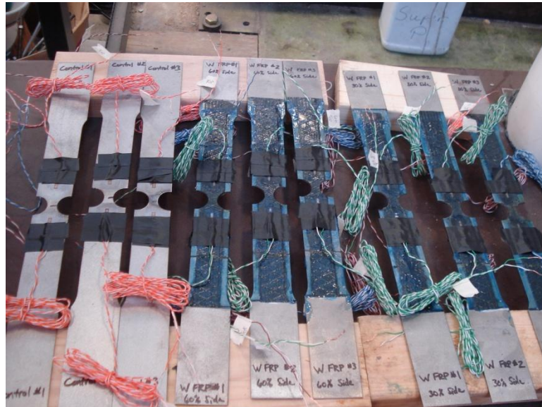
Figure 3.18. Wrinkle Coupon Set
