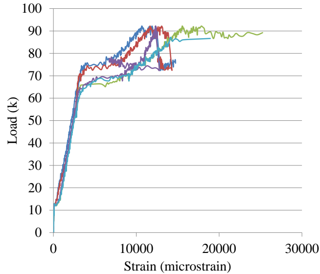
Figure 4.60. Load-Strain: Steel Rebar
