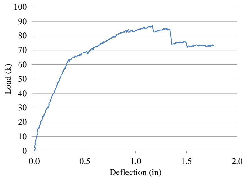
Figure 4.68. Load-Deflection: Beam 10
