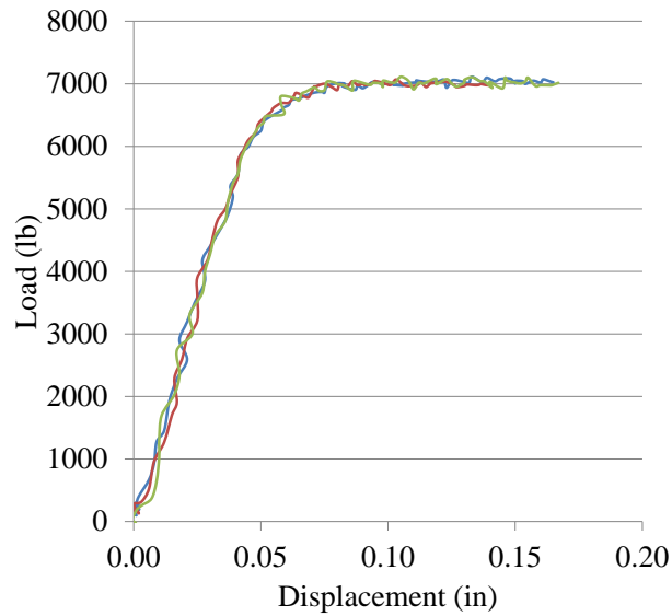
Figure 3.6. Load-Displacement: Control
