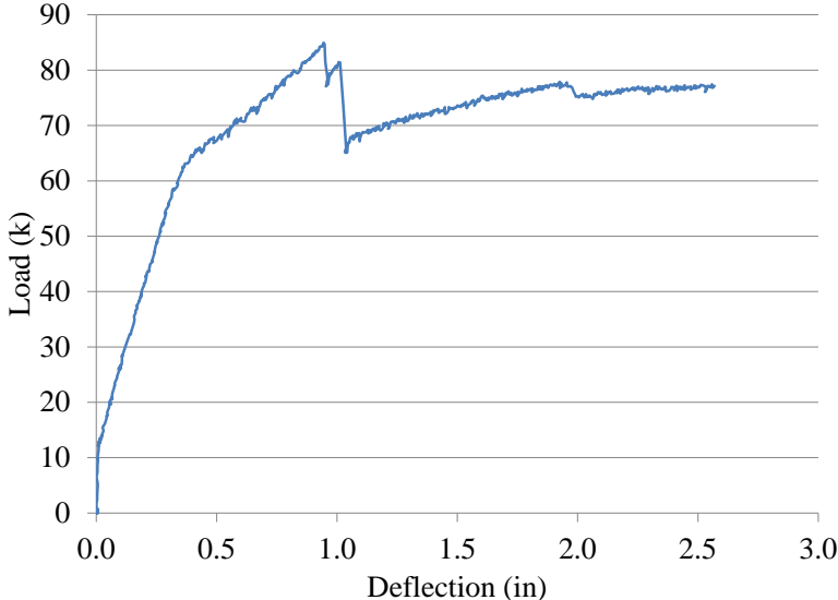
Figure 4.14. Load-Deflection: Beam 2
