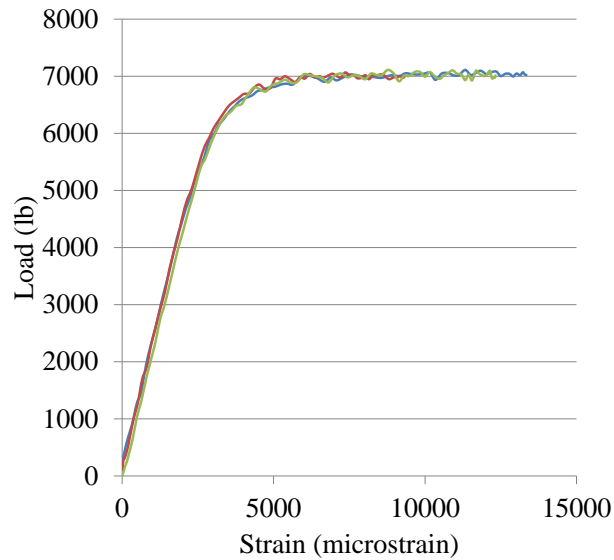
Figure 3.7. Load-Strain: Control
