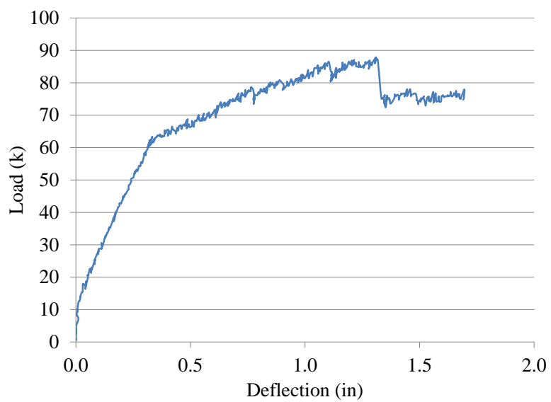
Figure 4.74. Load-Deflection: Beam 11
