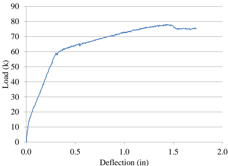
Figure 4.32. Load-Deflection: Beam 1
