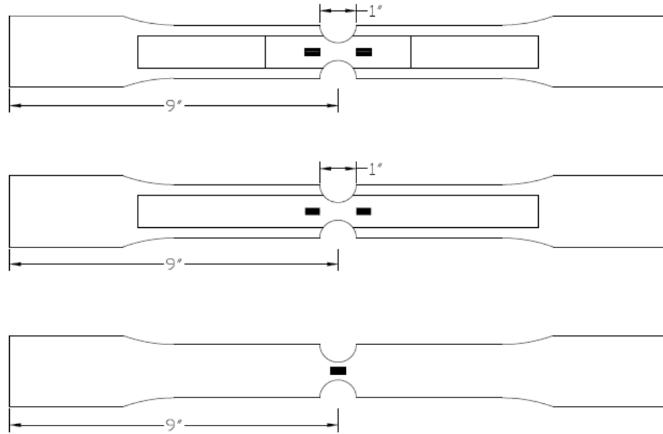
Figure 3.19. Wrinkle Strain Gage Locations: Preloaded, Non-Preloaded, Control
