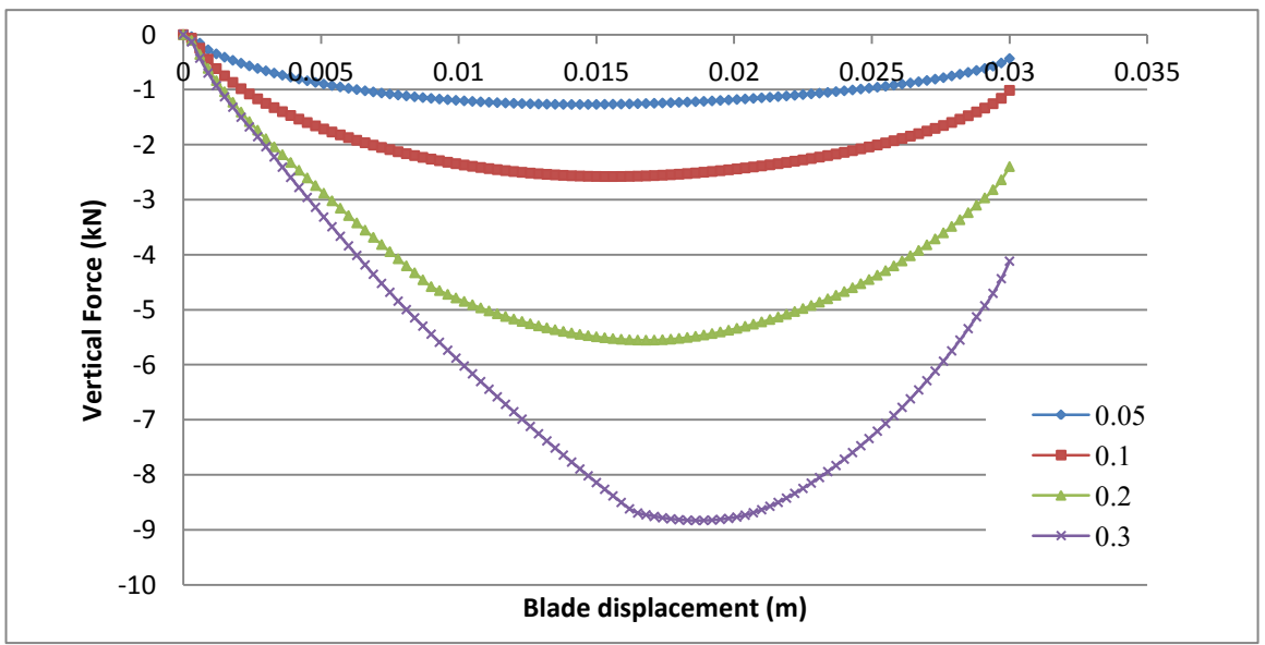
Figure 4.20 Effect of soil-metal coefficient of friction on vertical force
