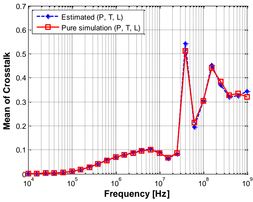
Figure 3.30. Mean value of crosstalk when varying load, twist and wire positions, for two circuits where inductive coupling dominates (RMS difference 4%).
