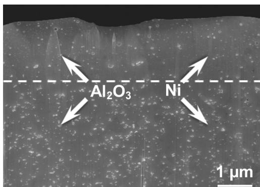
FIG. 11. SEM micrographs of the surface of the laser melted Ni/Al 2 O 3 nanocomposite at 0.18 mJ.
