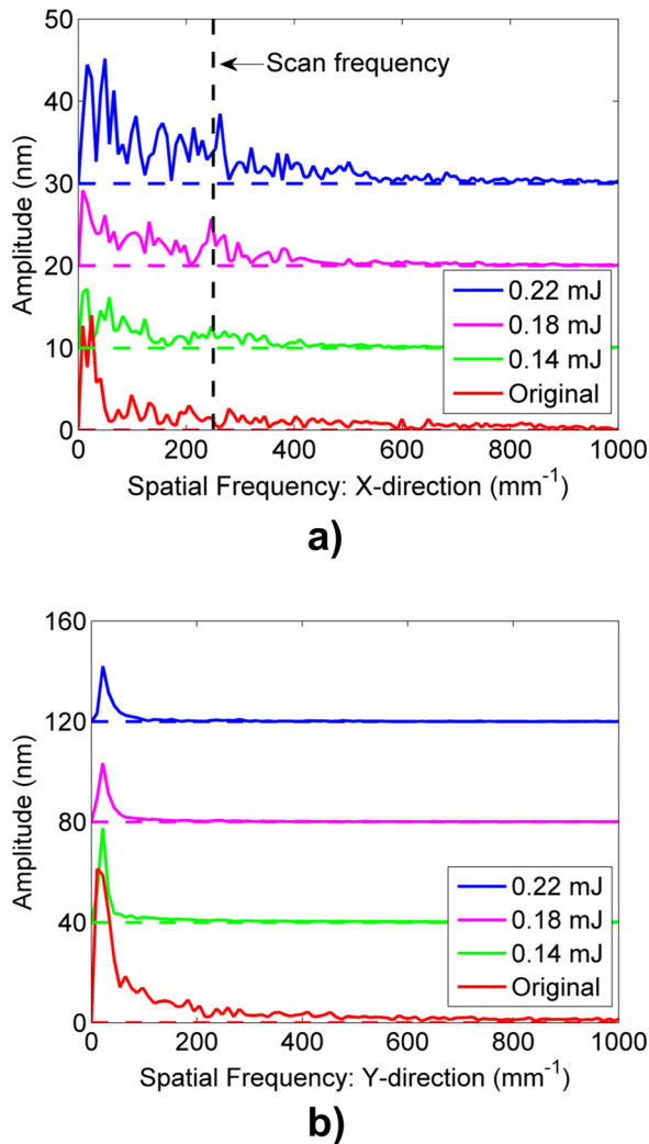
FIG. 10. Spatial frequency spectra of Ni/Al 2 O 3 surface before and after laser melting at various pulse energies: (a) X-direction and (b) Y-direction.
