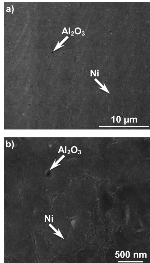
FIG. 12. SEM micrographs of the cross section of the laser melted Ni/Al 2 O 3 nanocomposite at 0.18 mJ at (a) low and (b) high magnifications.
