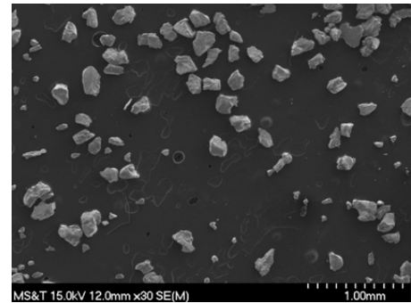
(c) Vanadium powder SEM image
