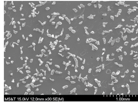
(b) Aluminum powder SEM image
