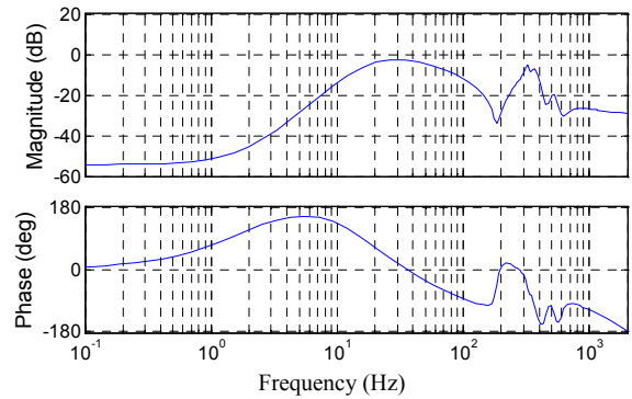
Fig. 6. Bode plot of \hat{P}(q) .
