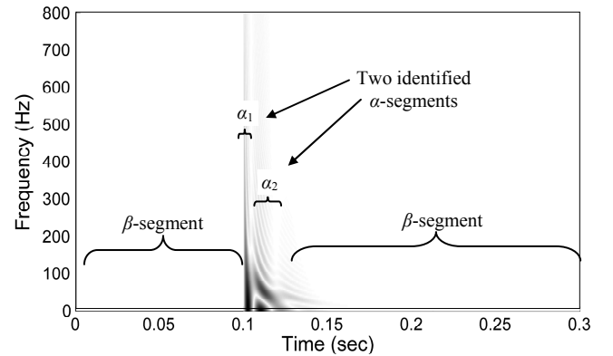
Fig. 2. Wigner-Ville time-frequency decomposition of e_0(k) .
