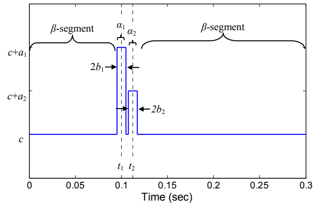
Fig. 3. Parameterized weighting profile, w(k) .
