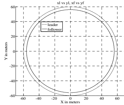
Fig. 4 Leader and follower trajectories
