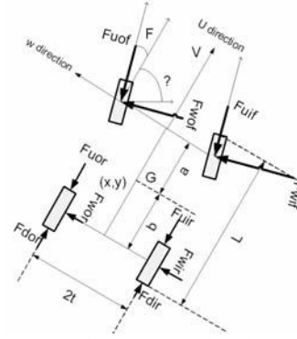
Fig.2 Free Body Diagram
