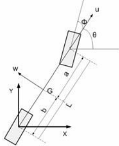
Fig.1 Bicycle model
