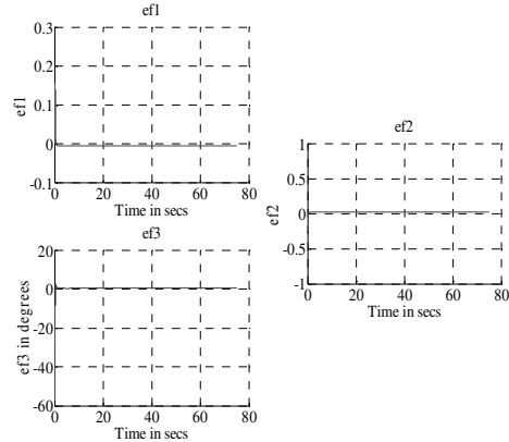
Fig. 5 Position and orientation errors
