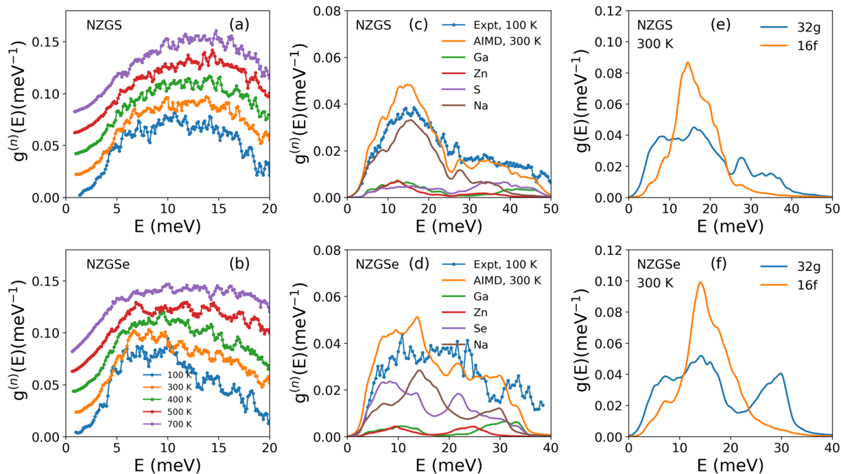
Fig. 2 (a and b) The measured temperature dependence of neutron-weighted PDOS of \text{Na}_3\text{ZnGaX}_4 ( X = \text{S}, \text{Se} ) compound using 26.0 meV incident neutron energy. (c and d) The calculated partial contribution of various species in \text{Na}_3\text{ZnGaX}_4 ( X = \text{S}, \text{Se} ) to total neutron weighted PDOS and compared with 100 K measured PDOS using 82.9 meV incident neutron energy. (e and f) The calculated partial phonon density of states of Na atoms at 32g and 16f Wyckoff sites.
