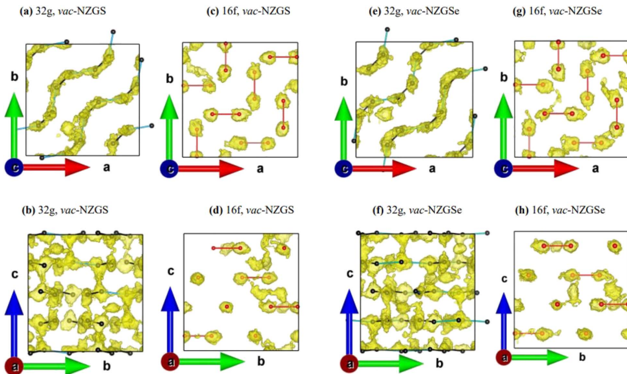
Fig. 6 The Na-Occupation probability-density (isosurface value \sim 0.001/\text{\AA}^3 ) of \text{Na}^+ initially occupied 16f and 32g Wyckoff sites, calculated using AIMD trajectories of vac -NZGS. (a–d) vac -NZGS, and (e–h) vac -NZGSe at 900 K. The Na at 32g sites are shown as black spheres, while the 16f sites are indicated by red spheres. The black and light blue bonds represent the first and second neighbour distances between Na's occupied at 32g sites. The first/second neighbour distances for Na at 32g sites are 3.2 \text{\AA} /4.06 \text{\AA} and 3.36 \text{\AA} /4.17 \text{\AA} , for NZGS and NaZGSe, respectively. The red bonds represent the first neighbour distance between Na's occupied at 16f sites. The first neighbour distances between Na at 16f sites are 4.25 \text{\AA} and 4.47 for NZGS and NaZGSe, respectively. Differences between the panels are described in the main text.
