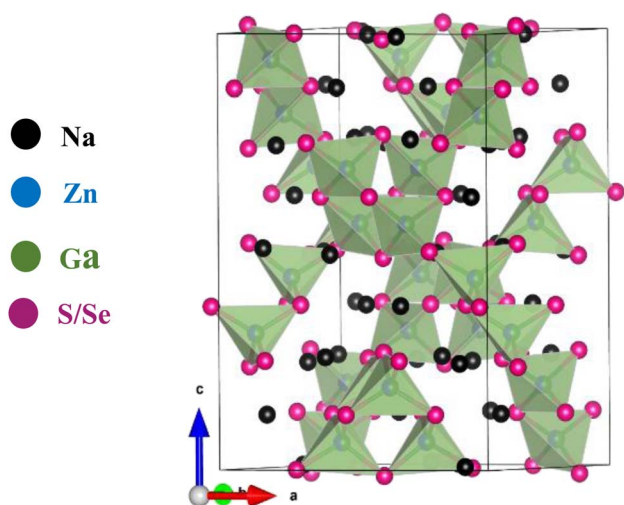
Fig. 1 The tetragonal crystal structure of \text{Na}_3\text{ZnGaX}_4 (body-centred tetragonal, space group I4_1/acd , Z = 16 ), where ( X = \text{S}, \text{Se} ). Zn and Ga occupy 32g Wyckoff sites with occupancies 0.5 : 0.5 and form the polyhedral unit \text{Zn/GaX}_4 . The room temperature lattice parameters of \text{Na}_3\text{ZnGaX}_4 ( X = \text{S/Se} ) are a = b = 12.925/13.43 Å and c = 18.623/19.15 Å.
