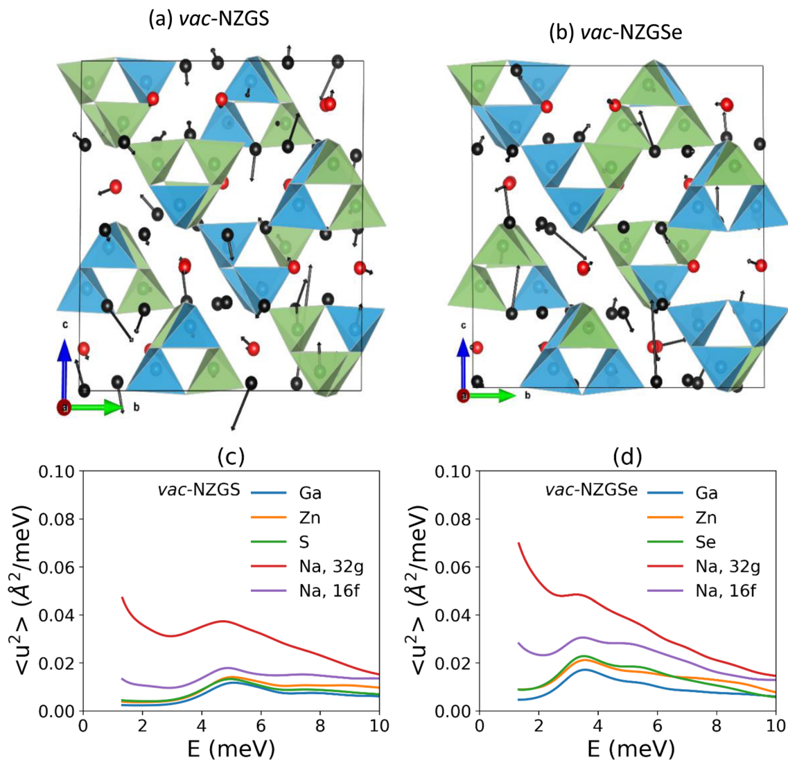
Fig. 3 (a and b) The calculated harmonic phonon eigenvectors of 32g and 16f Wyckoff sites Na atoms in the vacancy structure of \text{Na}_3\text{ZnGaX}_4 ( X = \text{S}, \text{Se} ). The Na at 32g sites is indicated by black spheres, while at 16f sites is shown by red spheres. The displacements pattern for S and Se compounds are shown for phonon modes of energy 5.8 meV. We have shown only half of the unit cell boundary along the a -axis for clarity. The \text{ZnX}_4 and \text{GaX}_4 polyhedral units are indicated by green and blue colors, respectively. (c and d) The calculated energy dependence of averaged phonon contribution to MSD at 900 K of \text{Na}_3\text{ZnGaX}_4 ( X = \text{S}, \text{Se} ).
