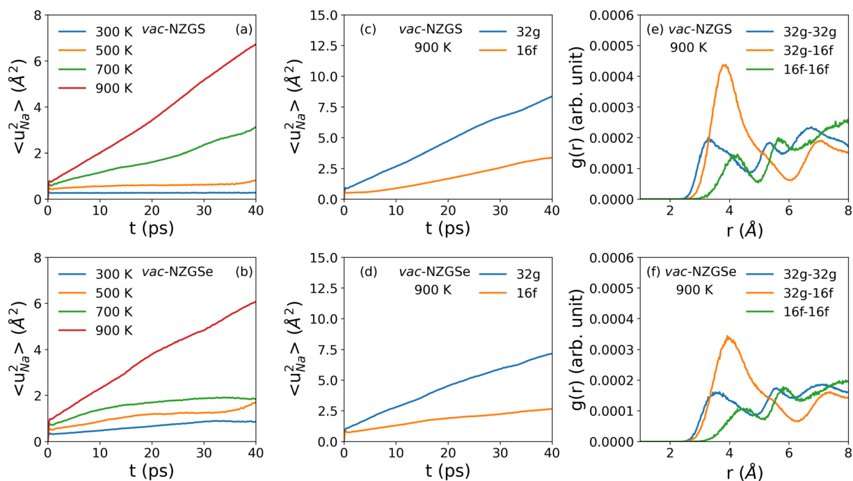
Fig. 5 (a and b) The calculated Na-MSD with 2% Na vacancy in \text{Na}_3\text{ZnGaX}_4 ( X = \text{S, and Se} ) at various temperatures using AIMD trajectories. (c and d) The calculated site specific Na-MSD between 32g-32g and 16f-16f Wyckoff sites in vac -NZGS and vac -NZGSe. (e and f) The calculated Na-Na PDF between Na at 16f and 32g Wyckoff sites of vac -NZGS and vac -NZGSe.
