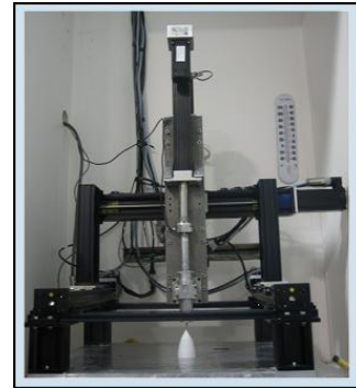
Figure 3. Freeze-form Extrusion Fabrication (FEF) Machine.
