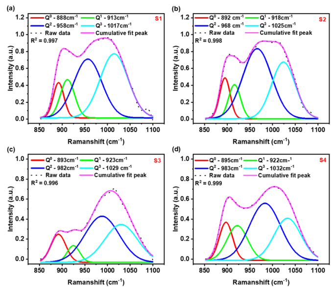
Fig. 6. Deconvoluted Raman spectra of 1400 °C synthetic fluxes for the Q region from 850-1100 \text{cm}^{-1} for sample 1 to sample 4. Four individual peaks were identified from all four samples. The cumulative fit peak (pink) has been compared with the raw data and provides the R square value to address the uncertainties.
