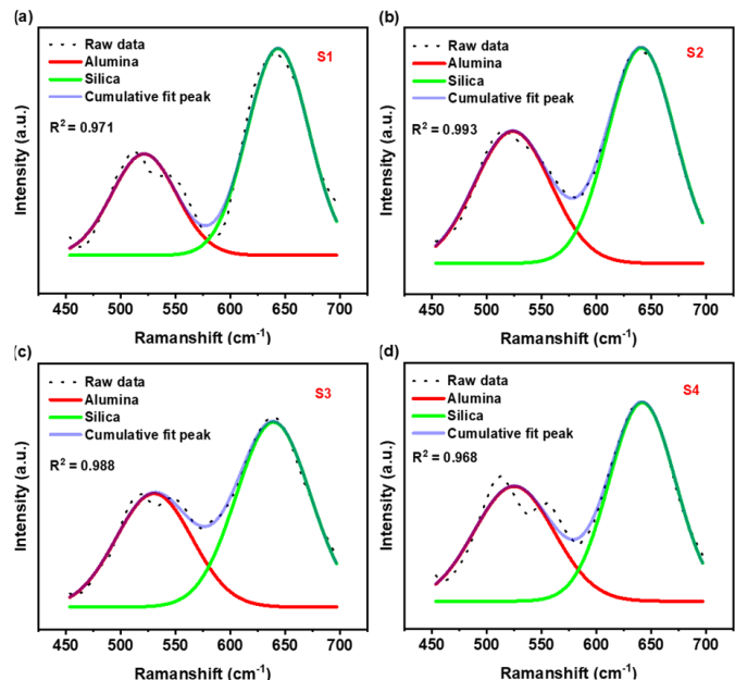
Fig. 4. Deconvoluted Raman spectra of 1400 °C synthetic fluxes for the alumina and silica regions for sample 1 to sample 4. The red and green peaks at 525 \text{cm}^{-1} and 645 \text{cm}^{-1} corresponded to alumina and silica.
