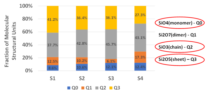
Fig. 8. Bar chart of the fraction of molecular structural units determined from deconvoluted Raman spectra of synthetic flux samples. The amount of monomer increases with the \text{CaO} (wt%) increase. The amount of sheet decreases with the \text{SiO}_2 (wt%) decrease. Sample 4 contains the highest amount of monomer has the highest basicity.
