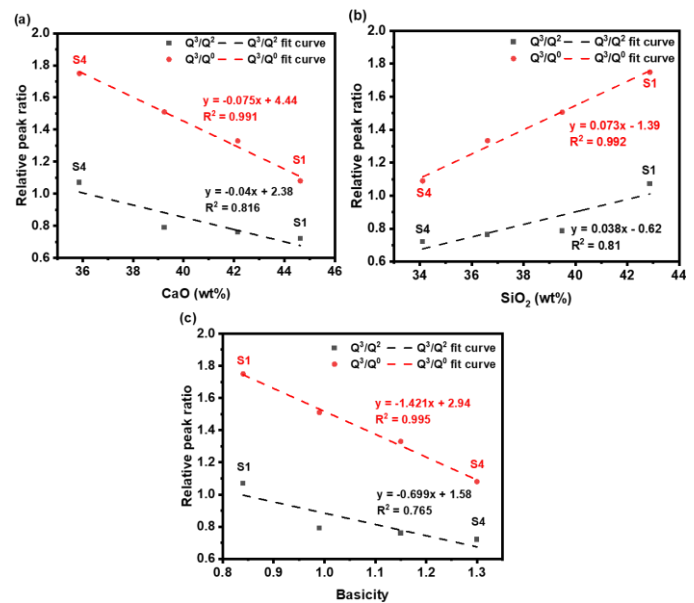
Fig. 7. Correlations of the Q region peak intensity ratio Q^3/Q^2 and Q^3/Q^0 to both flux chemical composition and basicity. (a) Q region peak intensity ratios of Q^3/Q^2 and Q^3/Q^0 versus \text{CaO} (wt%). (b) Q region peak intensity ratios of Q^3/Q^2 and Q^3/Q^0 versus \text{SiO}_2 (wt%). (c) Q region peak intensity ratios of Q^3/Q^2 and Q^3/Q^0 versus flux basicity.
