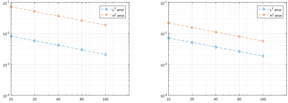
Figure 4.4. The ensemble simulations errors are O(1/\sqrt{J}) for \vec{u} (left) and \phi (right).
