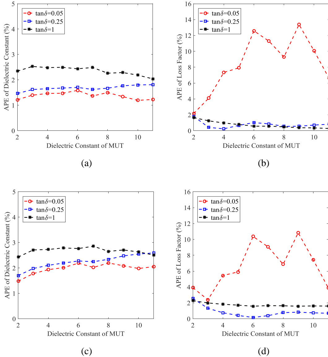
Figure 6. Errors for MUT with different complex permittivity, complex permittivity of reference material equals to k times the complex permittivity of room temperature distilled water: (a) results of dielectric constant error when k=0.8 , and (b) results of loss factor error when k=0.8 , (c) results of dielectric constant error when k=1.2 , and (d) results of loss factor error when k=1.2 .
