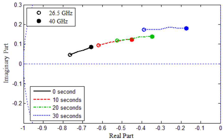
Figure 7. Measured Ka-band complex reflection coefficient of pig skin as a function of compounding burn episodes.
