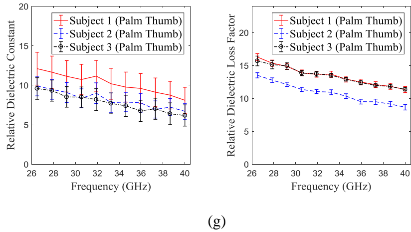
Figure 15. Relative dielectric constant and relative dielectric loss factor calculation results for: (a) forearm, (b) shoulder, (c) abdomen, (d) thigh, (e) calf, (f) palm (close to pinky), and (g) palm (close to thumb) (cont.).
