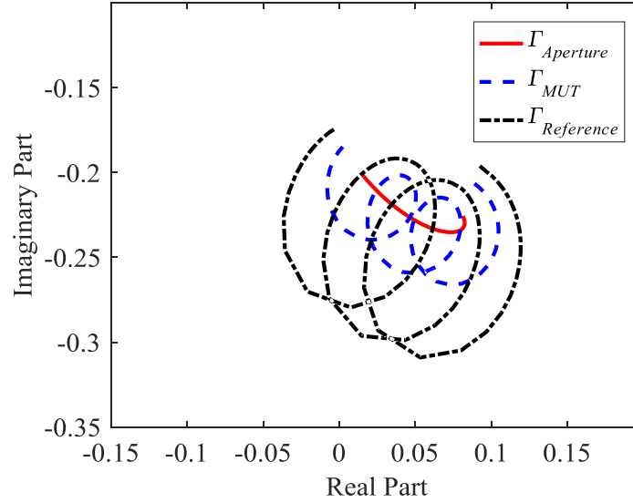
Figure 3. Calculated reflection coefficient at the waveguide probe aperture located at the center of the scanned plane when radiating into air, MUT and the reference material.
