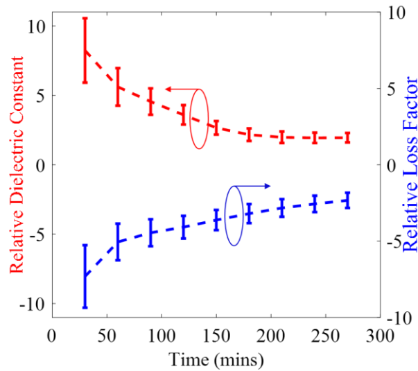
Figure 19. Calculated complex permittivity of wood sample over time.
