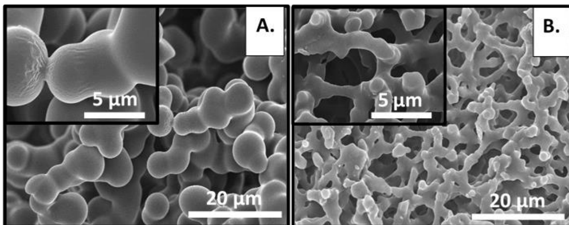
Figure 1.10. SEM images of (a). TEG based SMA and (b). TTEG based SMA.
