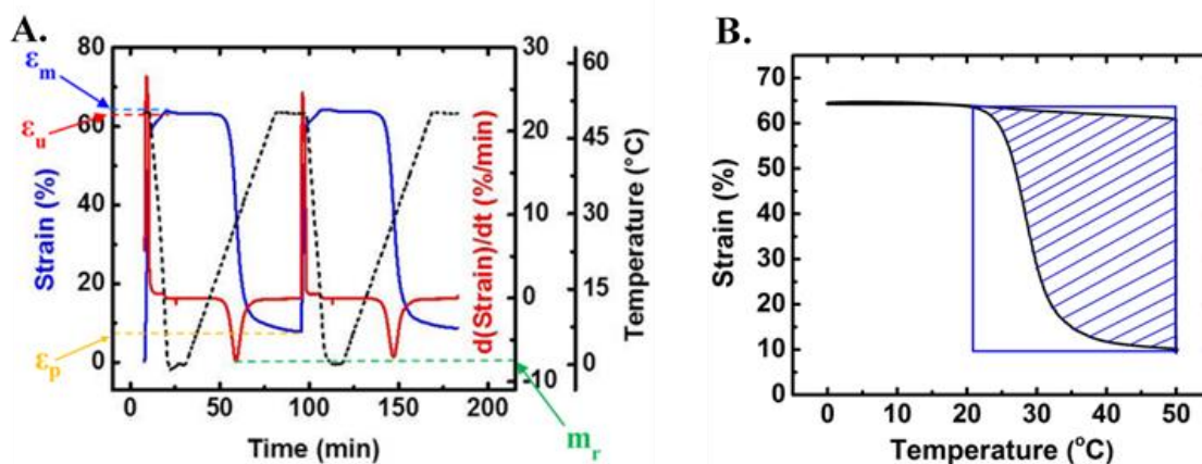
Figure 1.9. Projections of the entire 3D representation of Figure 1.8 to different planes in order to calculate the figures of merit of the shape memory effect. (a).
