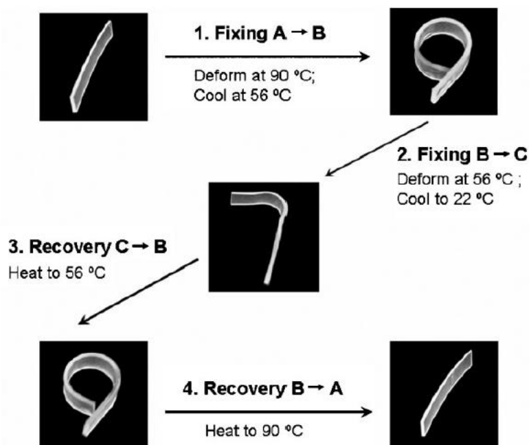
Figure 1.4. Photographs of a bilayer polymer demonstrating a triple shape memory effect.
