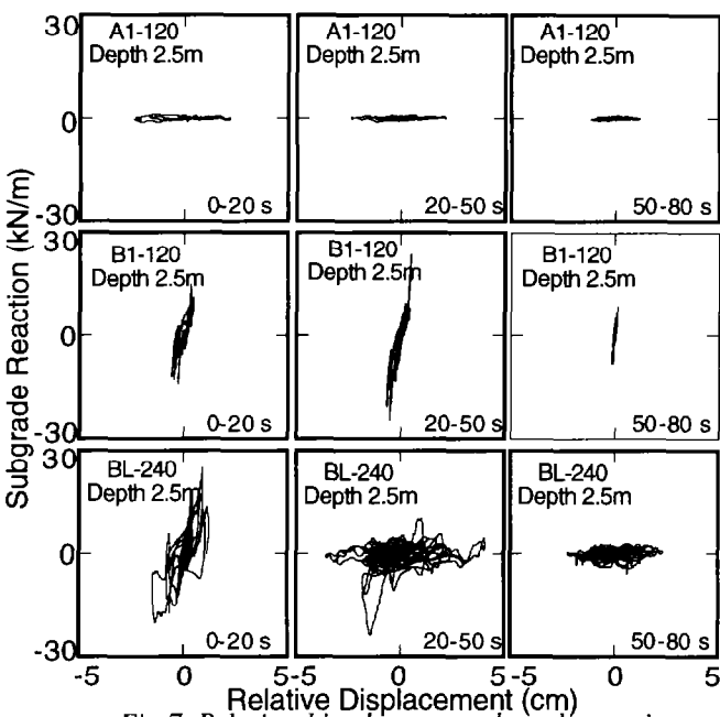
Fig.7. Relationships between subgrade reaction and relative displacement in A1-120, B1-120 and BL-240
