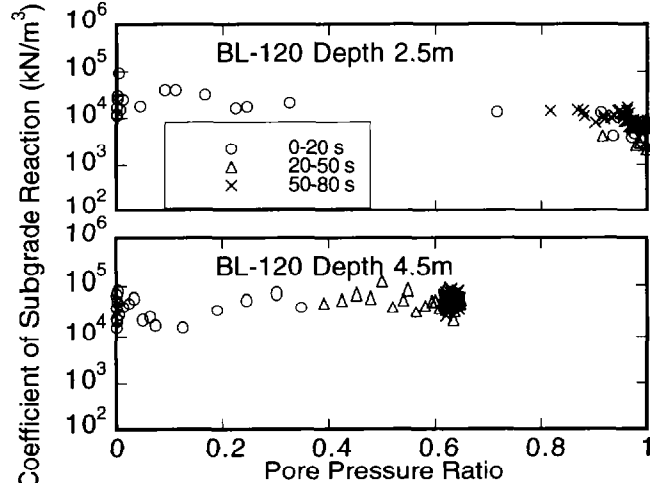
Fig.9. Relationships between coefficient of subgrade reaction and pore pressure ratio in BL-120
