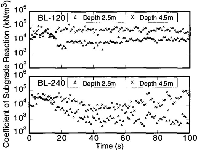
Fig.8. Change in coefficient of subgrade reaction with time in BL-120 and BL-240
