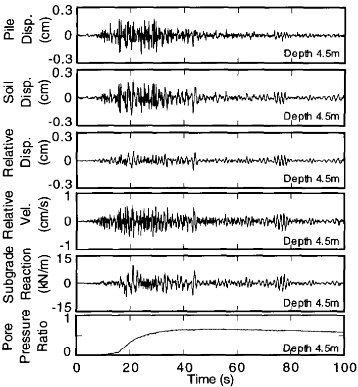
Fig.4. Time histories at 4.5m depth in BL-120
