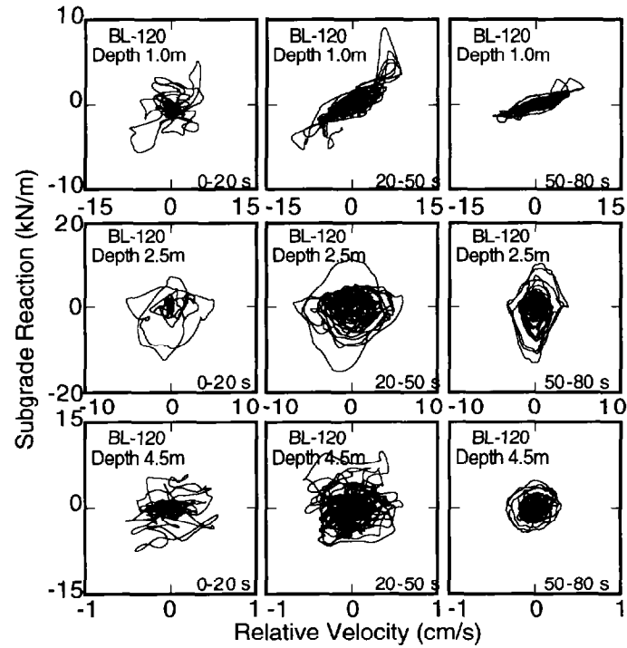
Fig.6. Relationships between subgrade reaction and relative velocity in BL-120
