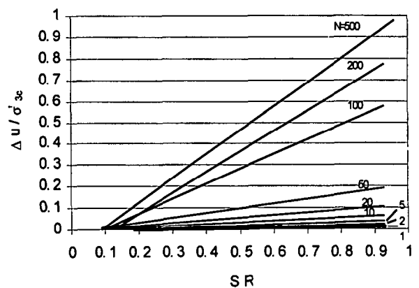
Fig. 8. Excess pore pressure ratio versus SR, for different cycle numbers.
