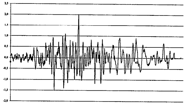
Fig 11. Horizontal component of accelerogram #7 ( \text{m/sec}^2 )
