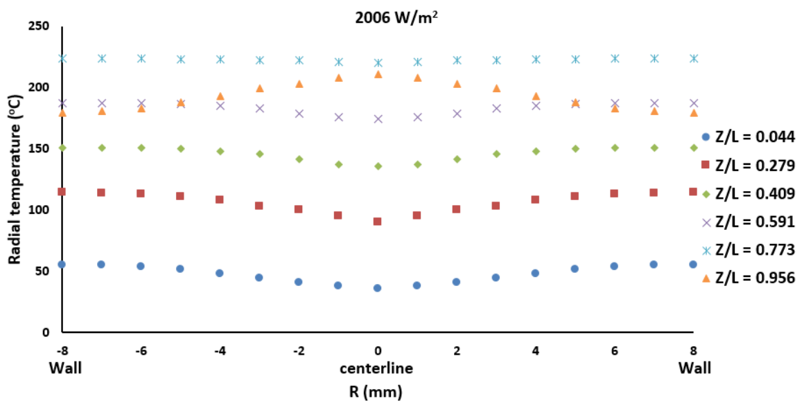
Fig. 14. Radial temperature distribution for helium at 2006 W/m 2 along the riser channel.
