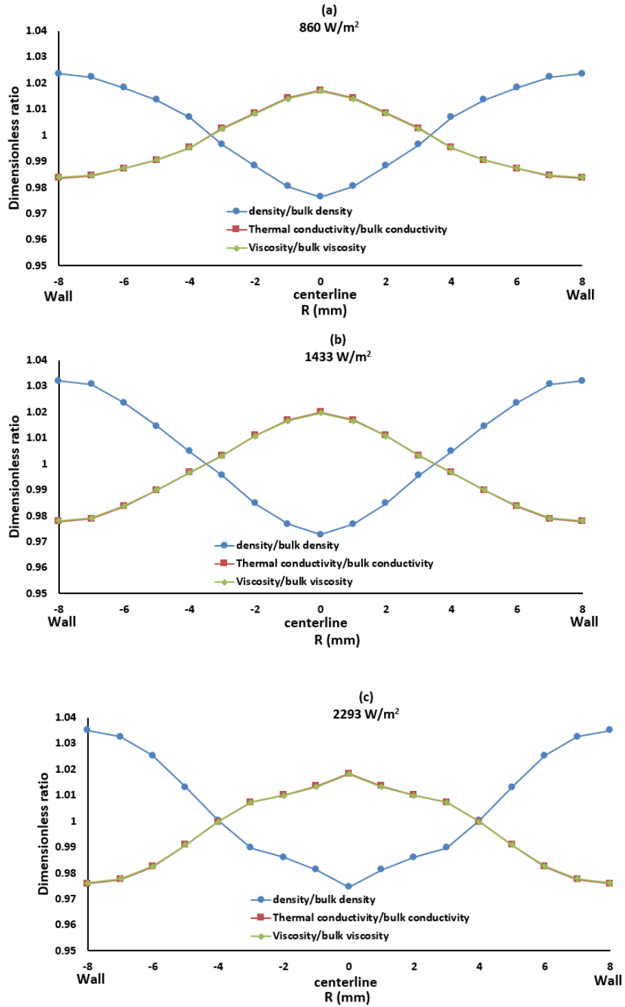
Fig. 19. Radial distribution of the physical properties at Z/L = 0.956 for different heat fluxes: (a) 860 \text{ W/m}^2 , (b) 1433 \text{ W/m}^2 , and (c) 2293 \text{ W/m}^2 along the riser channel.
