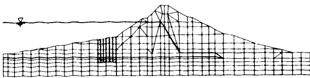
Fig. 26. Sardis Dam with Remediation Plug
