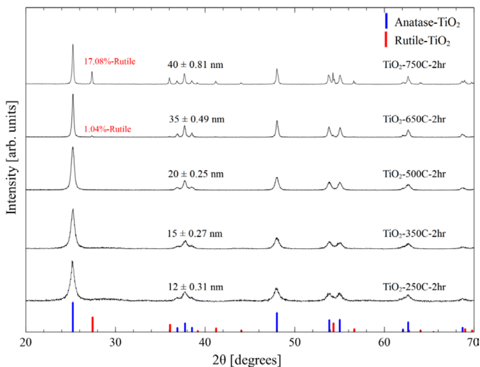
Figure 4.11. XRD patterns of \text{TiO}_2 nano particles prepared under \text{H}^+ concentration of 3 mol/L (pH = -0.48) environment and annealed at elevated temperatures from 250 °C to 750 °C.
