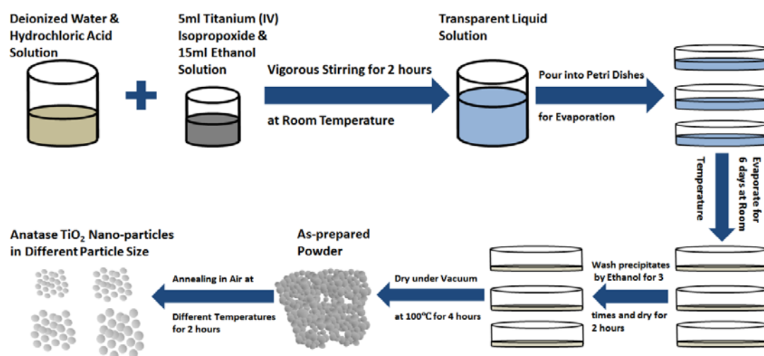
Figure 4.9. Synthesis of different sized anatase \text{TiO}_2 nano particles.
