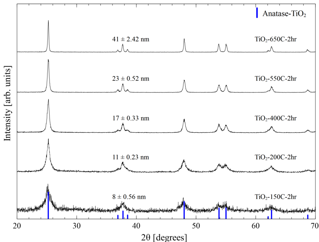
Figure 4.10. XRD patterns of TiO 2 nano particles prepared under H + concentration of 6 mol/L (pH = -0.78) environment and annealed at elevated temperatures from 150 °C to 650 °C.
