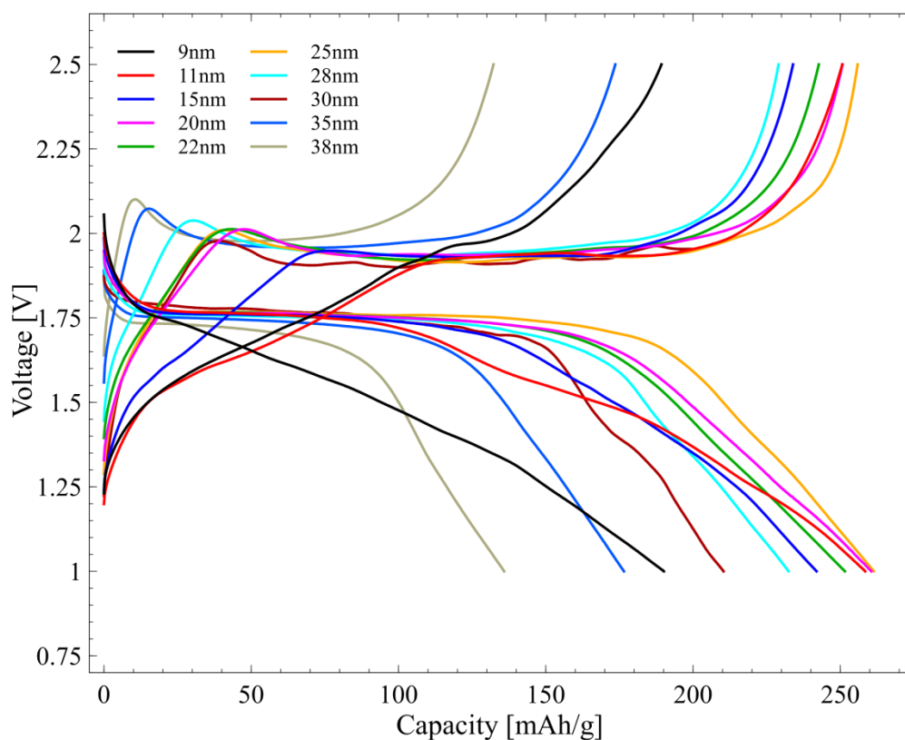
Figure 4.18. Charge/discharge voltage profiles at cycle#5 under C/3 of prepared anatase \text{TiO}_2 nano particles with particle size of 9, 11, 15, 20, 22, 25, 28, 30, 35 and 38 nm.
