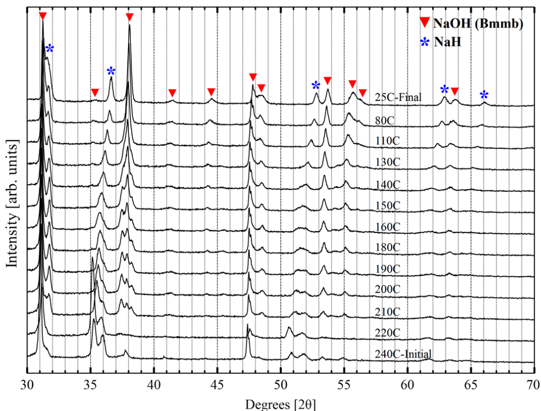
Figure 2.6. In-situ X-Ray diffraction data of cooling process for 40% NaH + 60% NaOH. Vertical guidelines (dotted lines) are given to emphasize the peak shifts.
