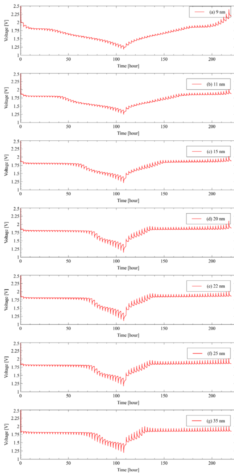
Figure 4.19. Galvanostatic intermittent titration technique (GITT) measurements for prepared anatase \text{TiO}_2 nano particles with particle size of (a) 9, (b) 11, (c) 15, (d) 20, (e) 22, (f) 25, and (g) 35 nm.
