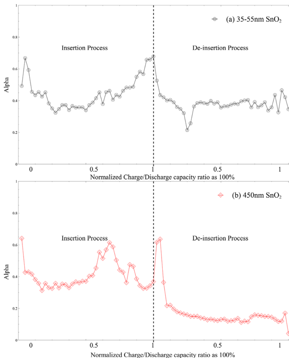
Figure 5.9. Fitted \alpha coefficient from the GITT measurements for commercial SnO 2 nano particles with particle size of (a) 35-55, and (b) 450 nm. Left half of each panel shows lithium insertion process and right half shows lithium de-insertion process.
