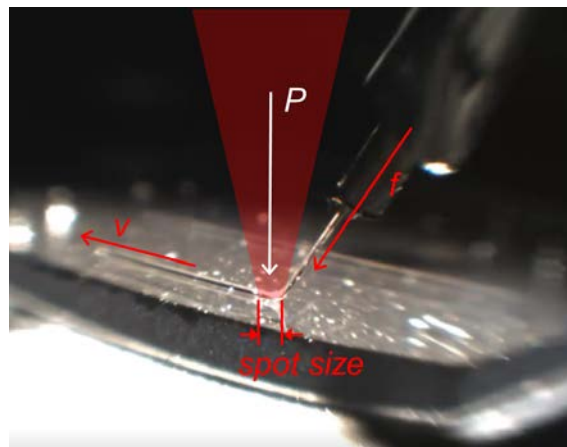
Fig. 2. Process parameters for fiber-printing specified for their effect on the deposited glass
