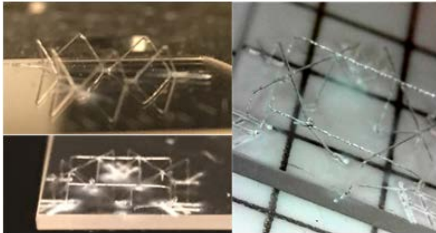
Fig. 7. Fiber truss in various stages of deposition
