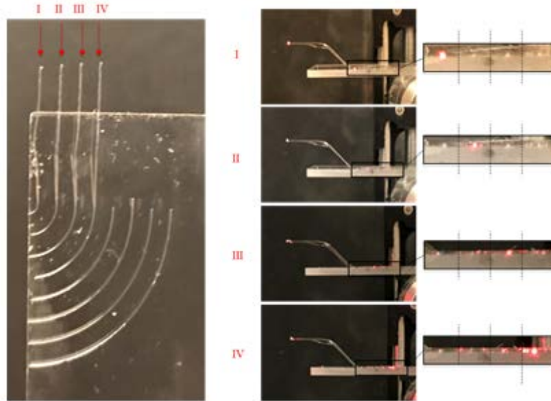
Fig. 9. Four adjacent waveguides demonstrating ability to isolate waveguide illumination
