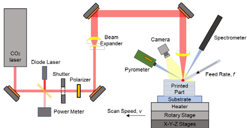
Fig. 1. Schematic of experimental platform
