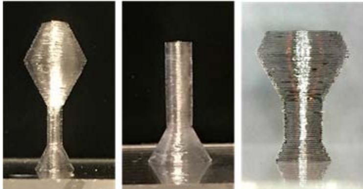
Fig. 5. Simple geometries deposited with quartz SMF
