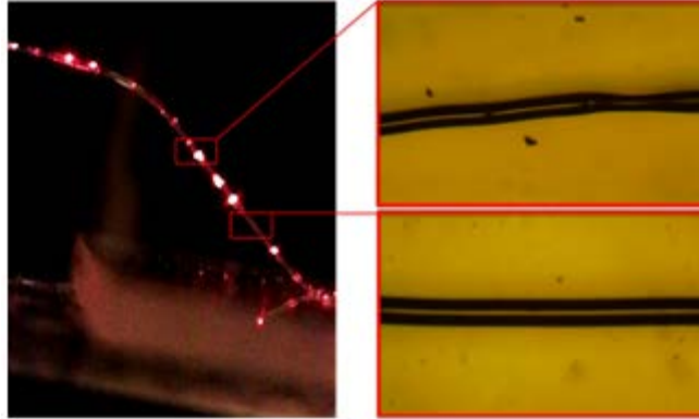
Fig. 10. Freestanding fiber observed under a microscope: Necking site which scatters light (top right), uniform segment which does not scatter light (bottom right)
