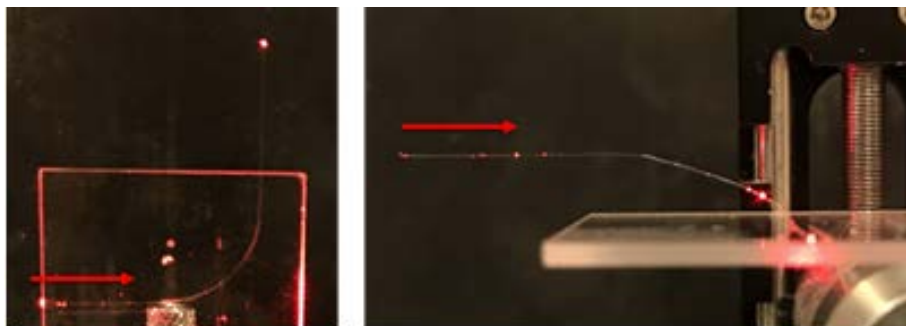
Fig. 8. HeNe laser beam guided through deposited quartz SMF fiber
