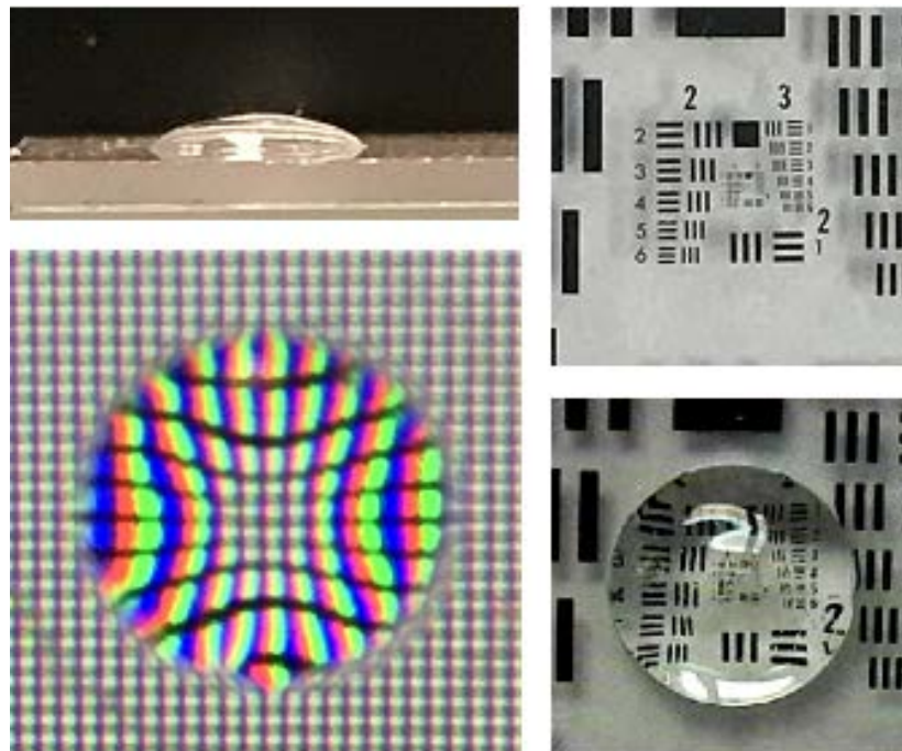
Fig. 4. Profile of spherical lens (top left), lens imaging pixels on LCD monitor (bottom left), AFRL resolution test chart with no lens (top right), AFRL resolution test chart imaged through spherical lens (bottom right)
