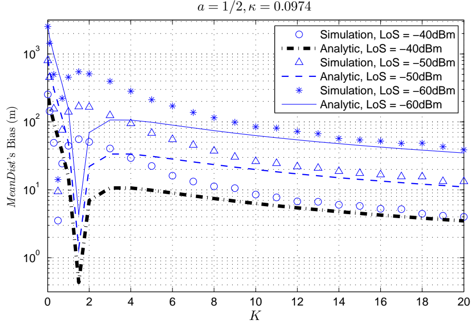
Figure 5. MeanDist's Bias
