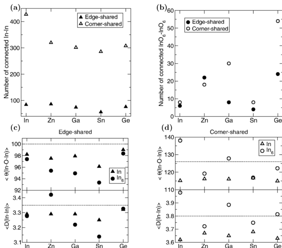
Figure 8. Number of edge-shared and corner-shared (a) In-In pairs and (b) \text{In}_6\text{-In}_6 pairs in amorphous In-O and In-X-O. Average In-In (triangle) or \text{In}_6\text{-In}_6 (circle) distance, in Å, and average In-O-In (triangle) or \text{In}_6\text{-O-In}_6 (circle) angle, in degrees, for the \text{InO}_x or \text{InO}_6 polyhedra connected via (c) edge-sharing or (d) corner-sharing in amorphous In-O and In-X-O. The horizontal dash line represents the corresponding values averaged for the second and third shells in crystalline \text{In}_2\text{O}_3 .
