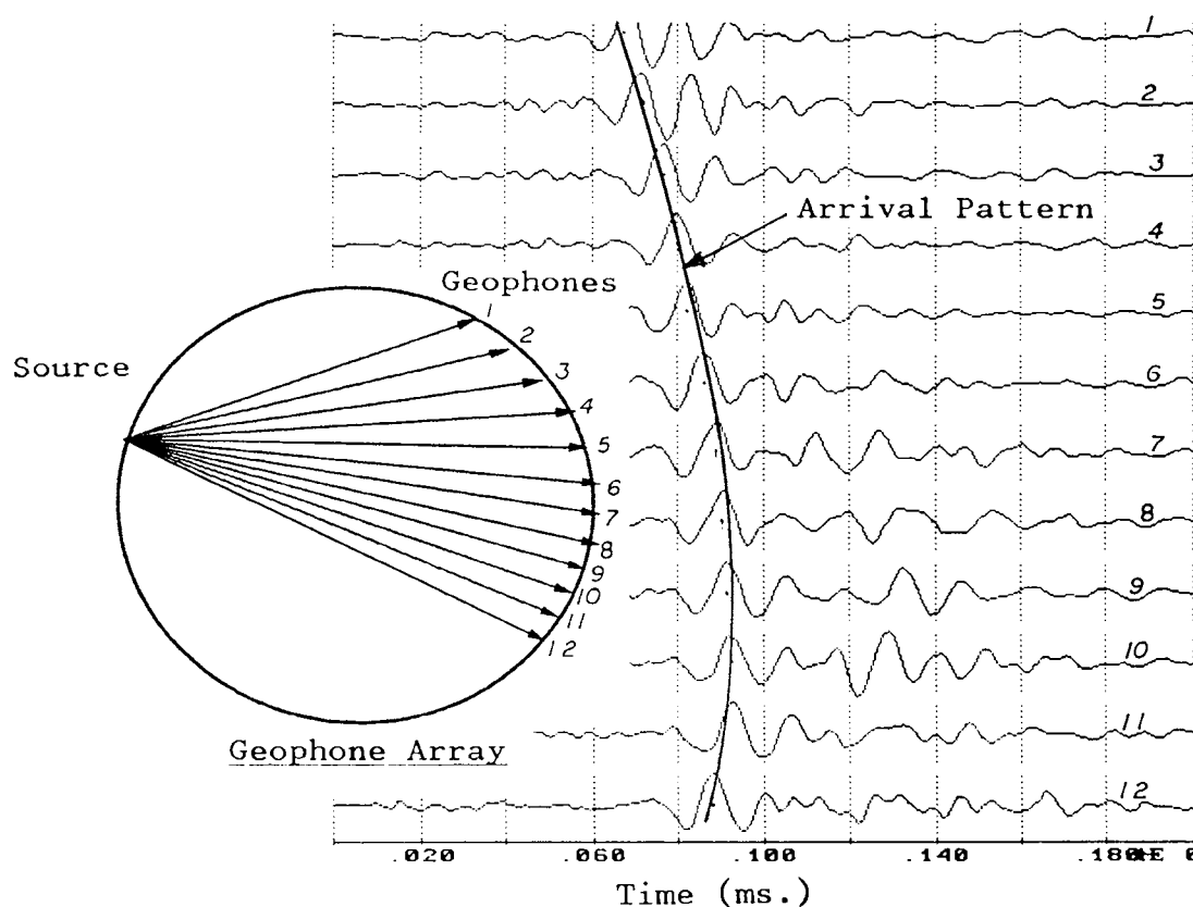
Figure 7 - Wave Arrival Pattern for Typical Geophone Array
