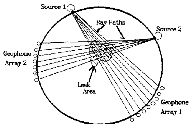
Figure 2 - Detection of Leakage using Multiple Geophone Arrays
