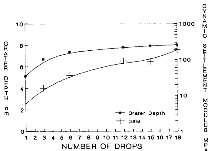
Figure 6 - Crater Depth and DSM vs Number of Drops.
