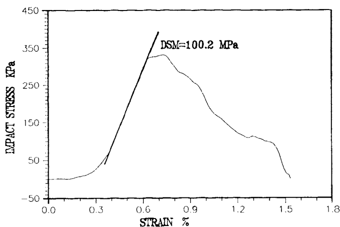
Figure 5 - Impact Stress vs Strain, Test 21, Drop 12.
