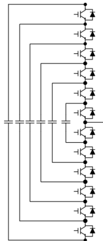
Figure 1.6. Flying capacitor multilevel topology
