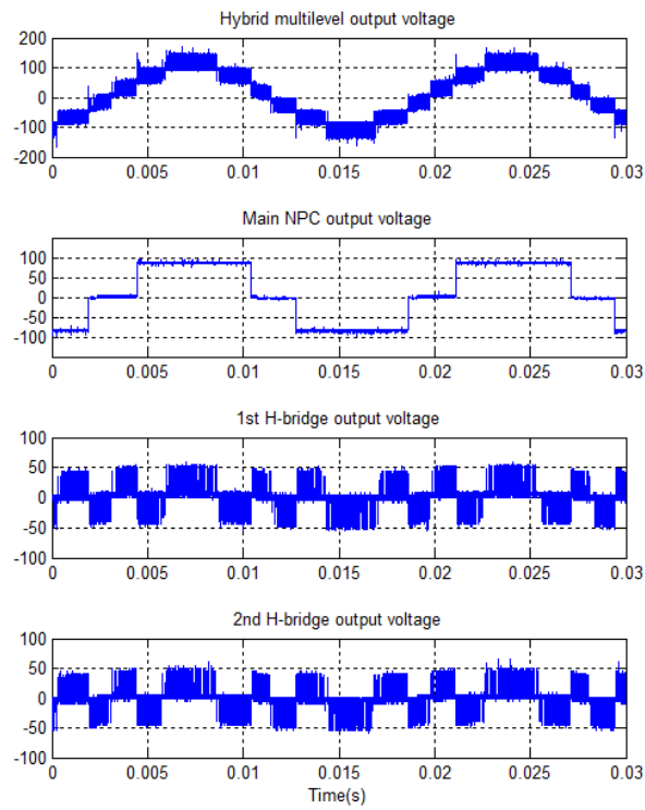
Figure 2. Experimental results explaining hybrid modulation method
