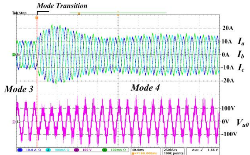
Figure 11. Transient responses of grid current and hybrid multilevel phase voltage output when voltage feedback loop is activated with V_{DC\_ref}=200V (from mode 3 to mode 4).
