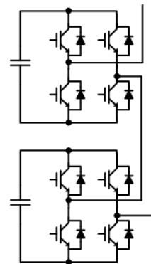
Figure 1.7. Cascaded H-bridge multilevel topology
