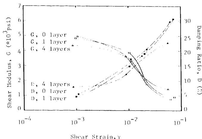
Fig. 9 Shear Modulus and Damping Ratio Versus Shear Strain Relationship for Cyclic Triaxial Test at 45-psi Confining Pressure
