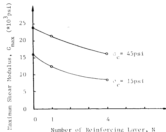
Fig. 11 Maximum Shear Modulus Versus Number of Reinforcing Layer Relationship
