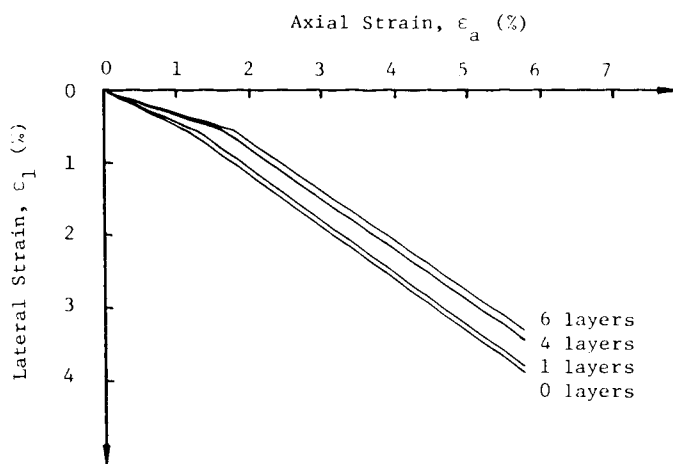
Fig. 6 Approximate Lateral Strain Versus Axial Strain Relationship at 45-psi Confining Pressure
