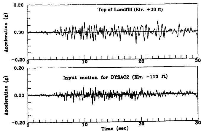
Fig. 6. Acceleration-Time Histories Predicted by SHAKE for Pier 300 East Dike Site
