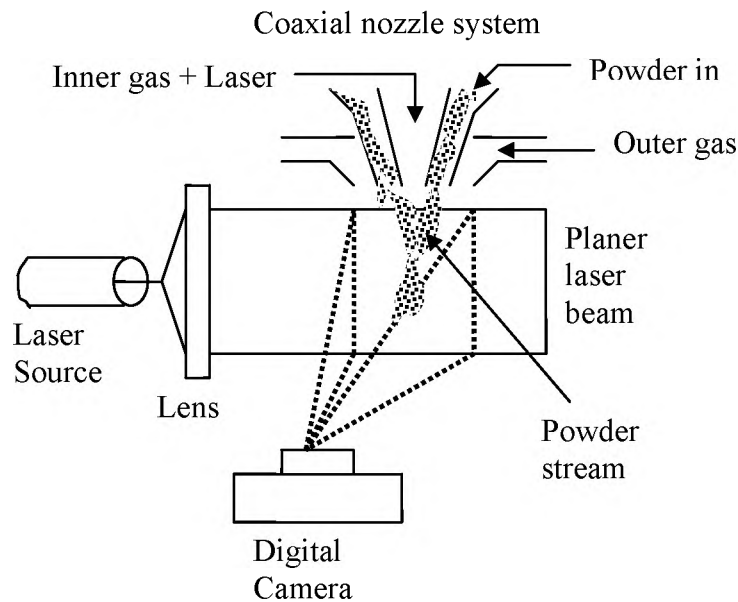
Figure 1: Experimental arrangement
