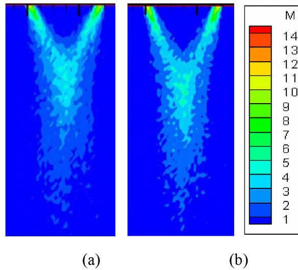
Figure 7: Simulation results: (a) 45° setting, (b) 60° setting
