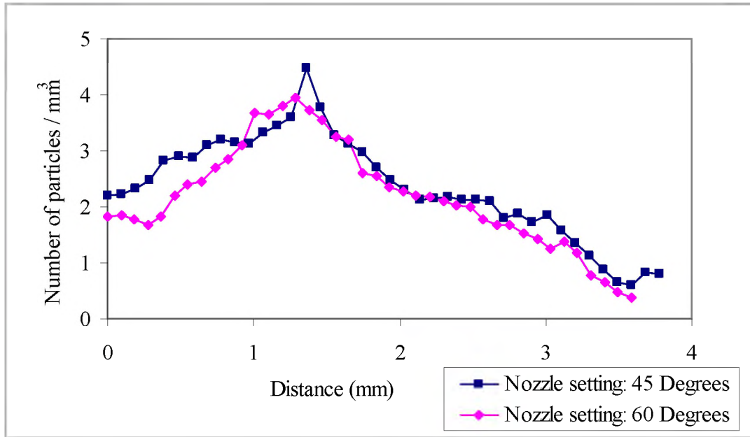
Figure 9: Radial distribution obtained with simulation method
