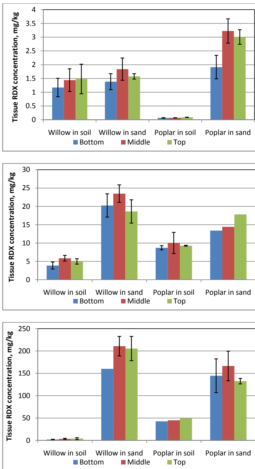
Figure G.1 Stem RDX Concentration in Small Scale Experiment (3 dosing levels)
