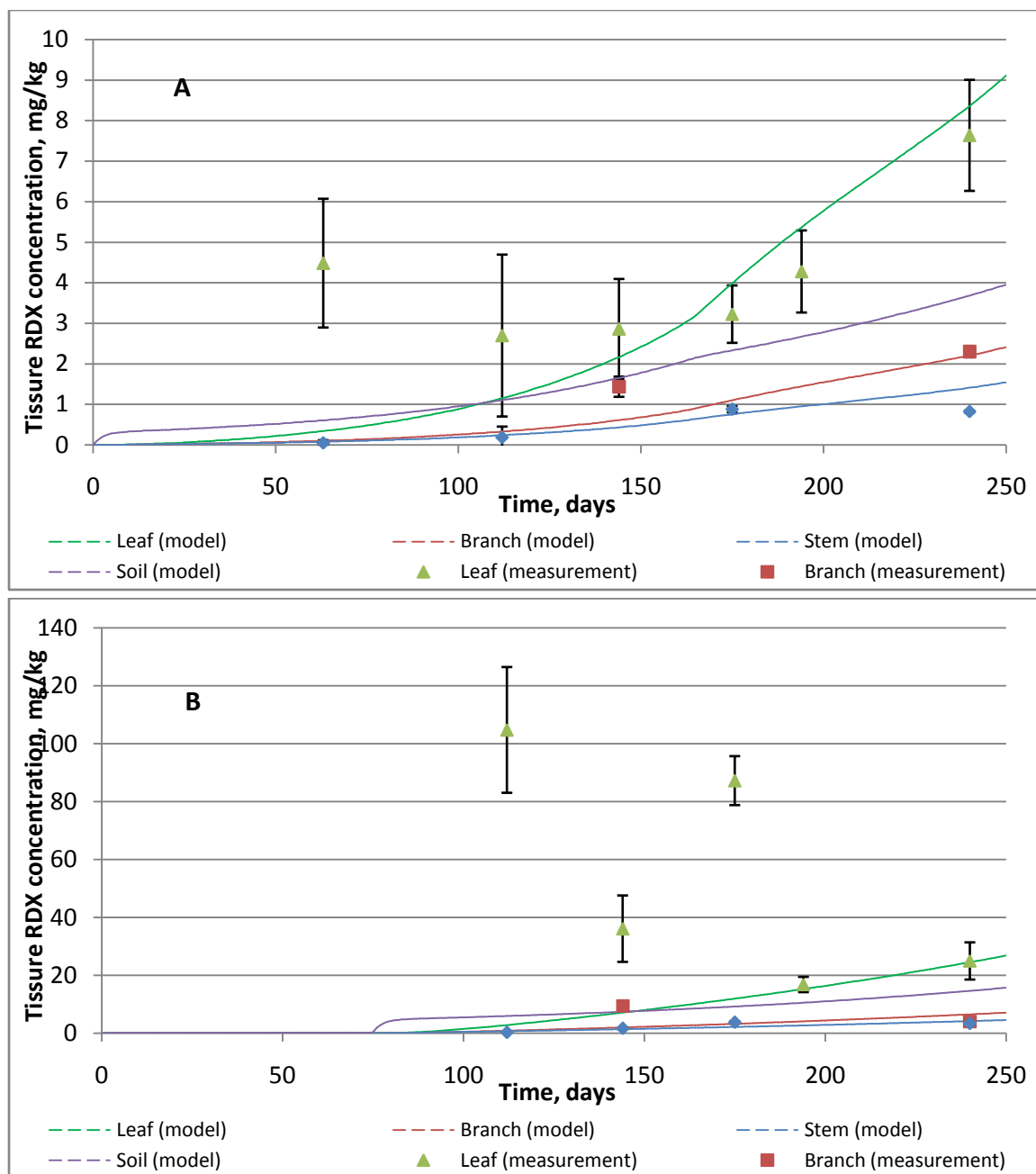
Figure J.1 Model Prediction and Experiment Measurement Comparisons: RDX, Large Scale Tree Experiment
