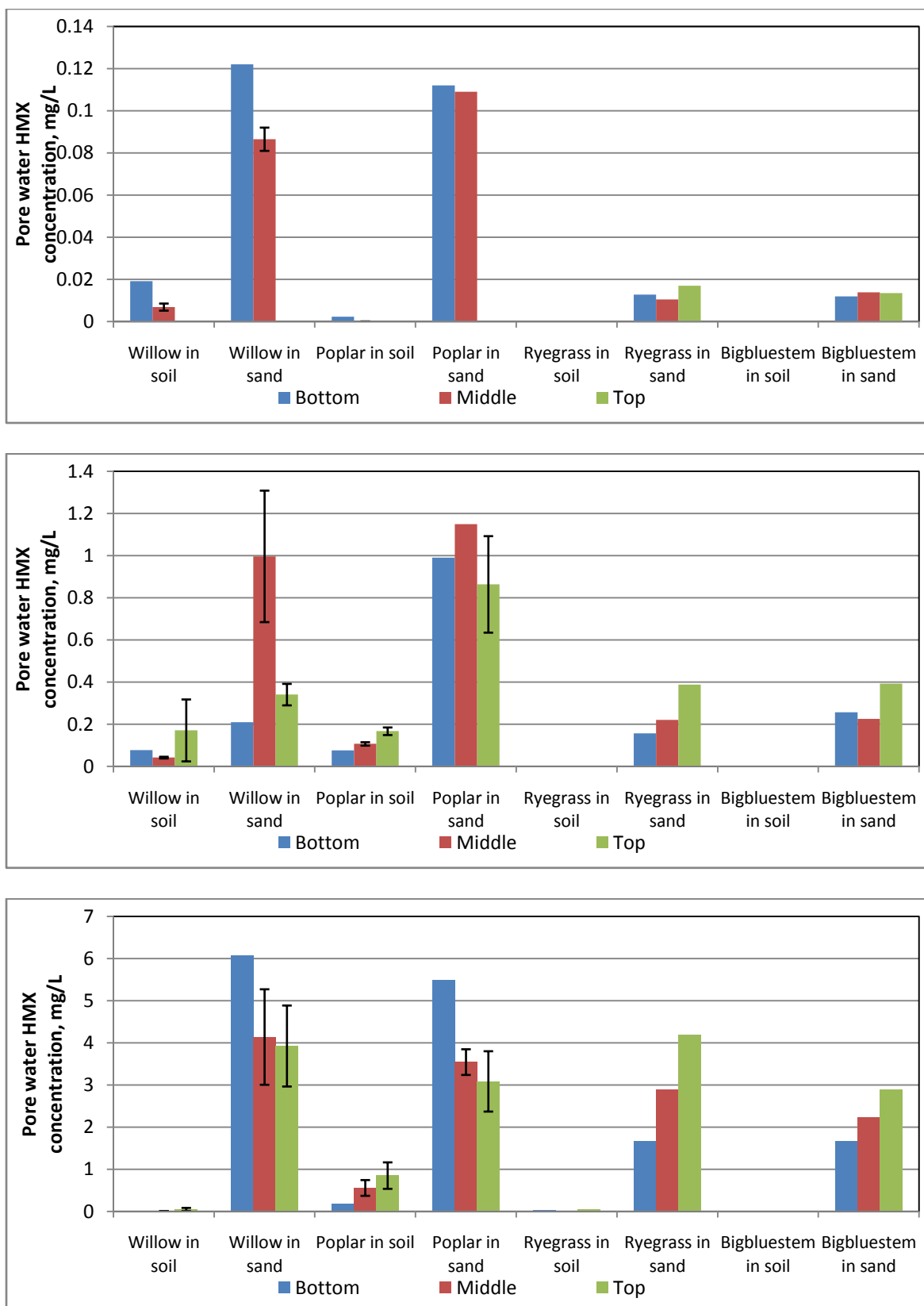
Figure D.10 Pore Water RDX Concentration Spatial Distribution
