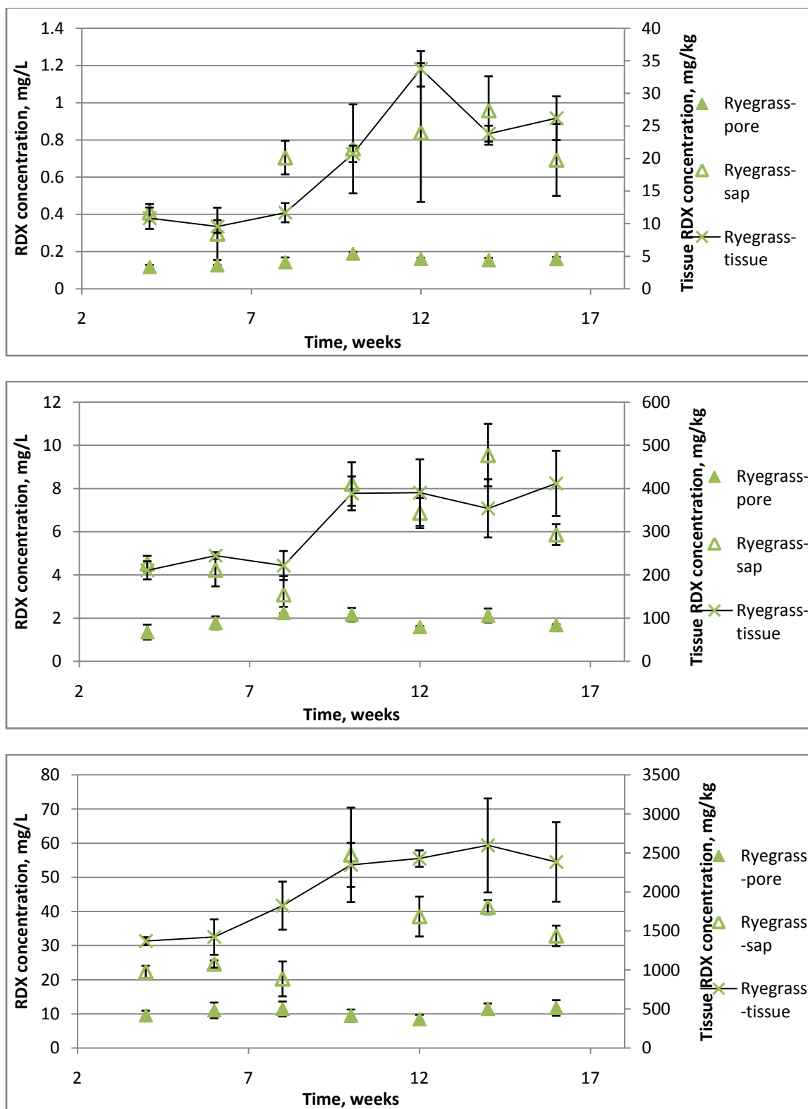
Figure 5.9 Ryegrass Tissue RDX Concentration (Based on DW), Low/Med/High
