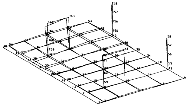
Fig. 7 Tilting Mode Shape
