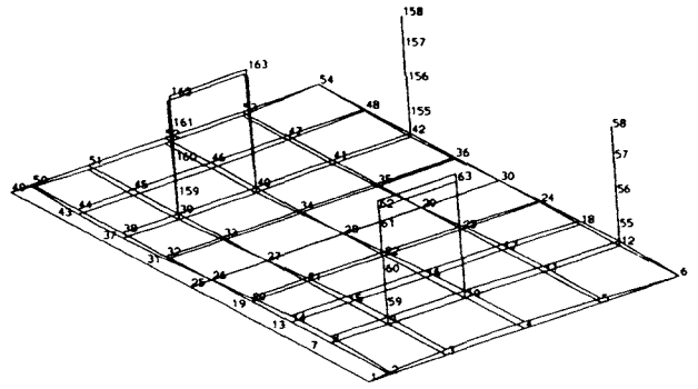
Fig. 6 Vertical Mode Shape
