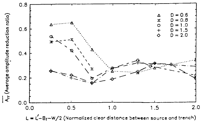
Fig. 4: Effect of Normalized Distance between Source and Trench for B_f=1.0
